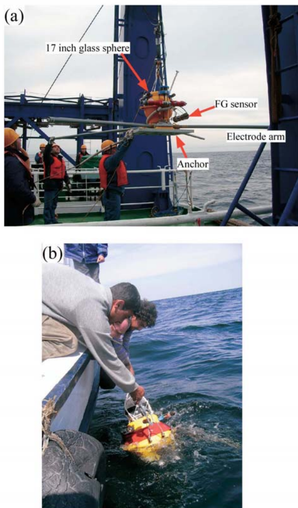
Fig. 3 (a) Deployment of the developed OBEM instrument. (b) Photograph of the recovery operation using a small fishing boat.
