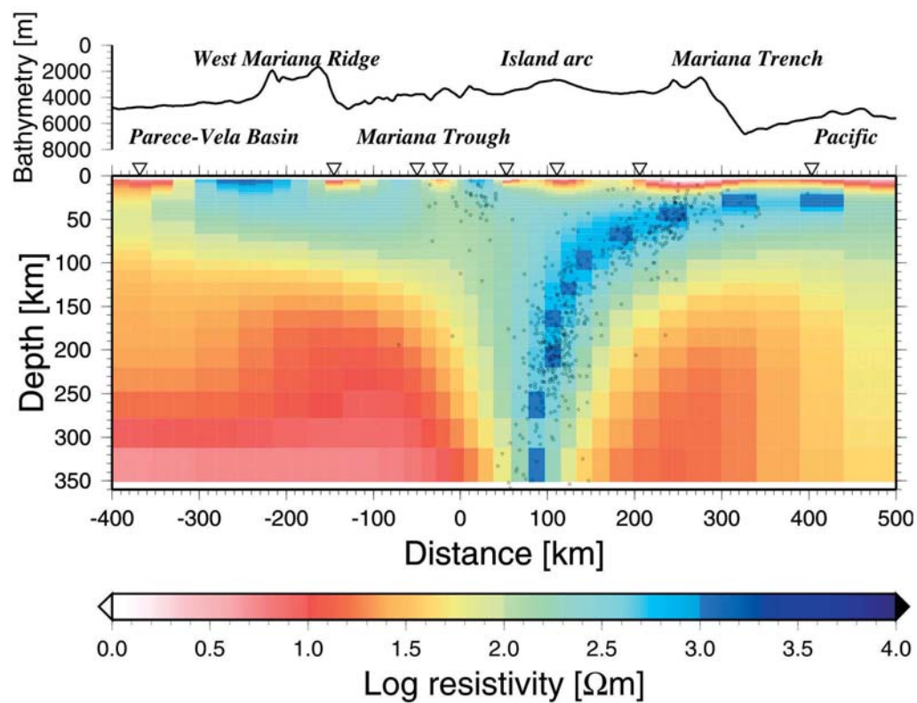
Fig.7 Two-dimensional model of the upper mantle electrical conductivity beneath the central Mariana area. Inversed triangles indicate the OBEM site locations. Dots are hypocenters. Bathymetric profile along the survey line is plotted on the top. After Baba et al. (2005).
