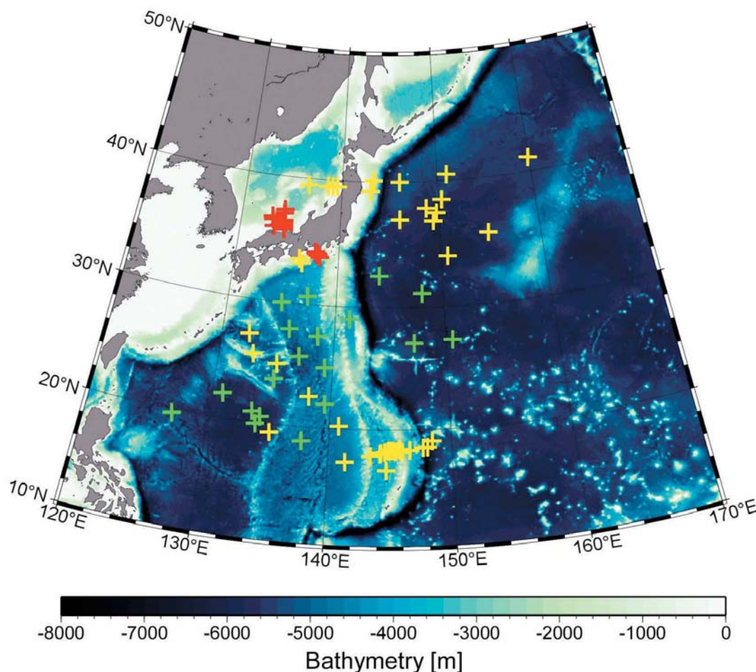
Fig. 1 All EM sites near Japan. Red crosses show Ocean Bottom Electro-Magnetic (OBEM) sites surveyed using new small OBEMs and OBEs. OBEM sites surveyed by the Stagnant Slab Project are shown as green crosses. Yellow ones show EM sites that were corrected by related project.
