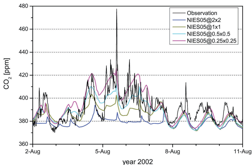
Fig. 6 Results of NIES05 at four kinds of resolutions at Tsukuba ( 36.05^{\circ}\text{N} , 140.13^{\circ}\text{E} ) 200m high tower, which is in close proximity of megacity Tokyo ( 35.66^{\circ}\text{N} , 139.75^{\circ}\text{E} ), and is occasionally under the influence of strong anthropogenic sources (an episode of up to about 70 ppm on 5 th afternoon). An offset of 373 ppm is added to the model values for comparison with observations. The model sampling grids are located at ( 37^{\circ}\text{N} , 141^{\circ}\text{E} ), ( 36.5^{\circ}\text{N} , 140.5^{\circ}\text{E} ), ( 36.25^{\circ}\text{N} , 140.25^{\circ}\text{E} ) and ( 36.13^{\circ}\text{N} , 140.13^{\circ}\text{E} ) in 2\times 2^{\circ} , 1\times 1^{\circ} , 0.5\times 0.5^{\circ} and 0.25\times 0.25^{\circ} model resolutions, respectively.
