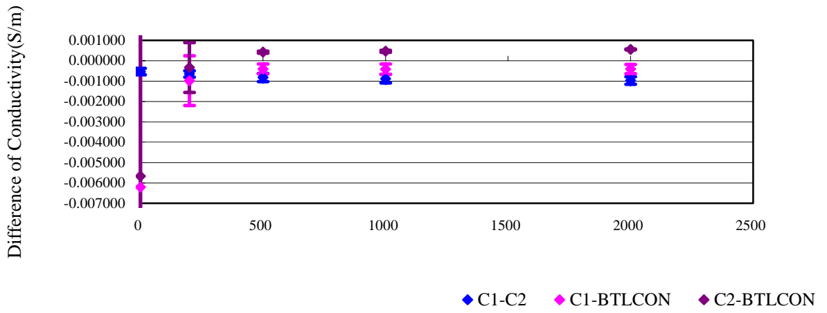
Fig. 2.2.1-3 Pressure dependence of Conductivity
