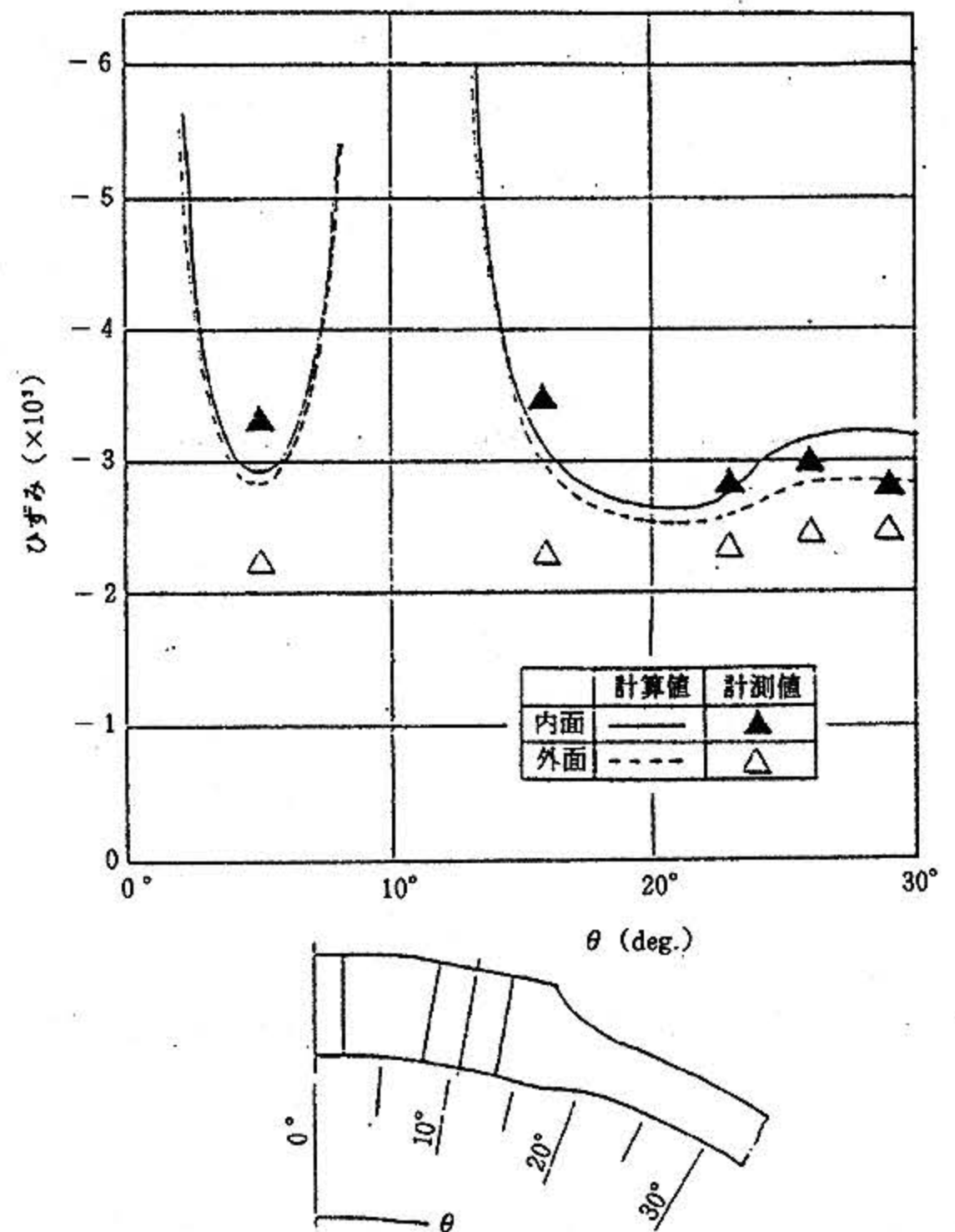
図14 集合電線貫通金物近傍緯線方向ひずみ分布 (外圧 680 kgf/cm²) Fig.14 Latitudinal Strain Distribution Around Viewport Coaming
