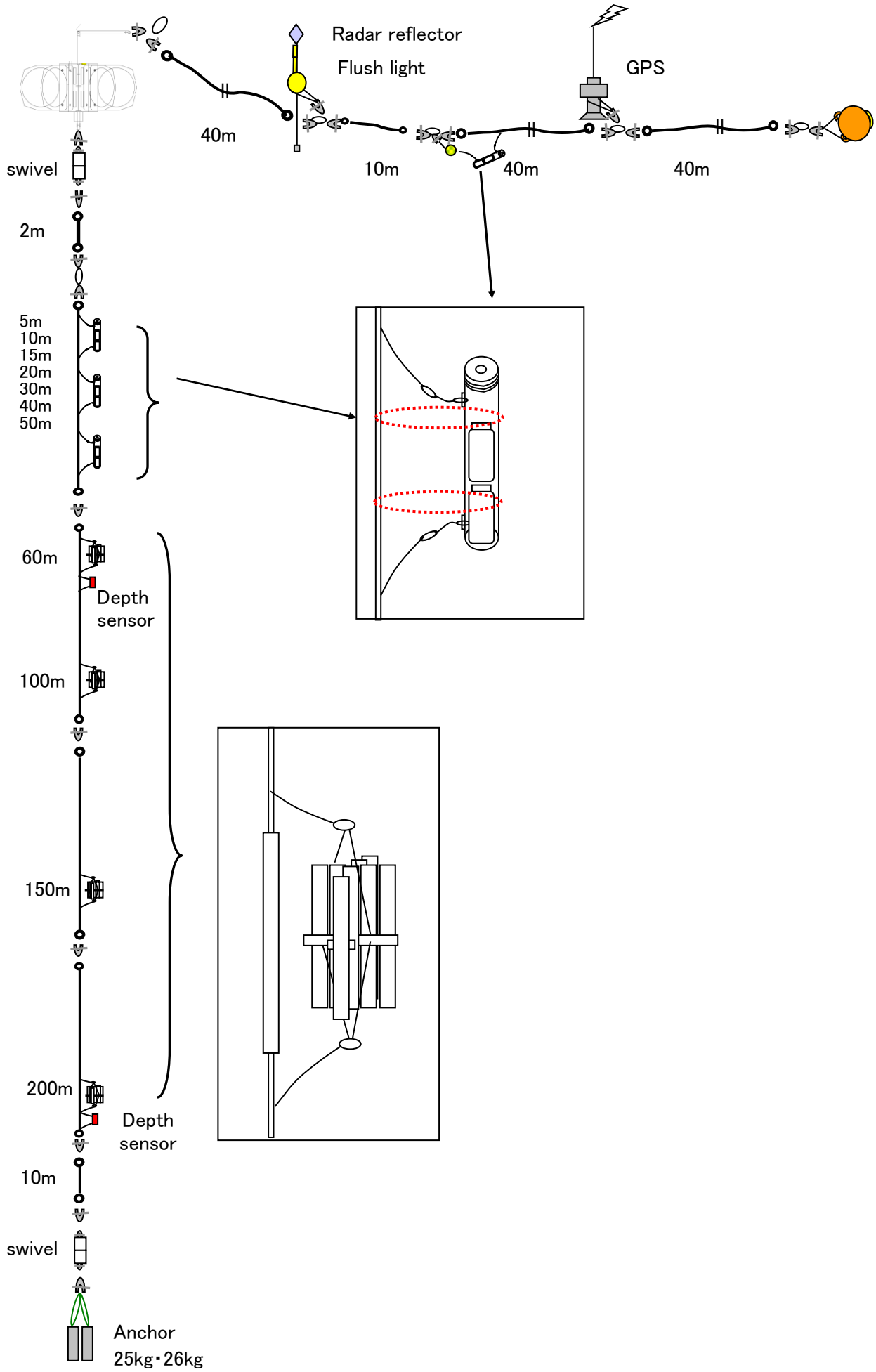
Drifting mooring system
