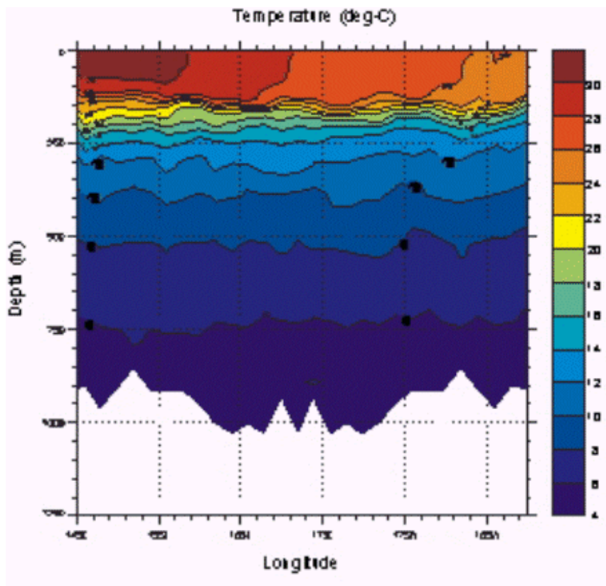
Fig.2 Vertical Section of Temperature (by XCTD)
