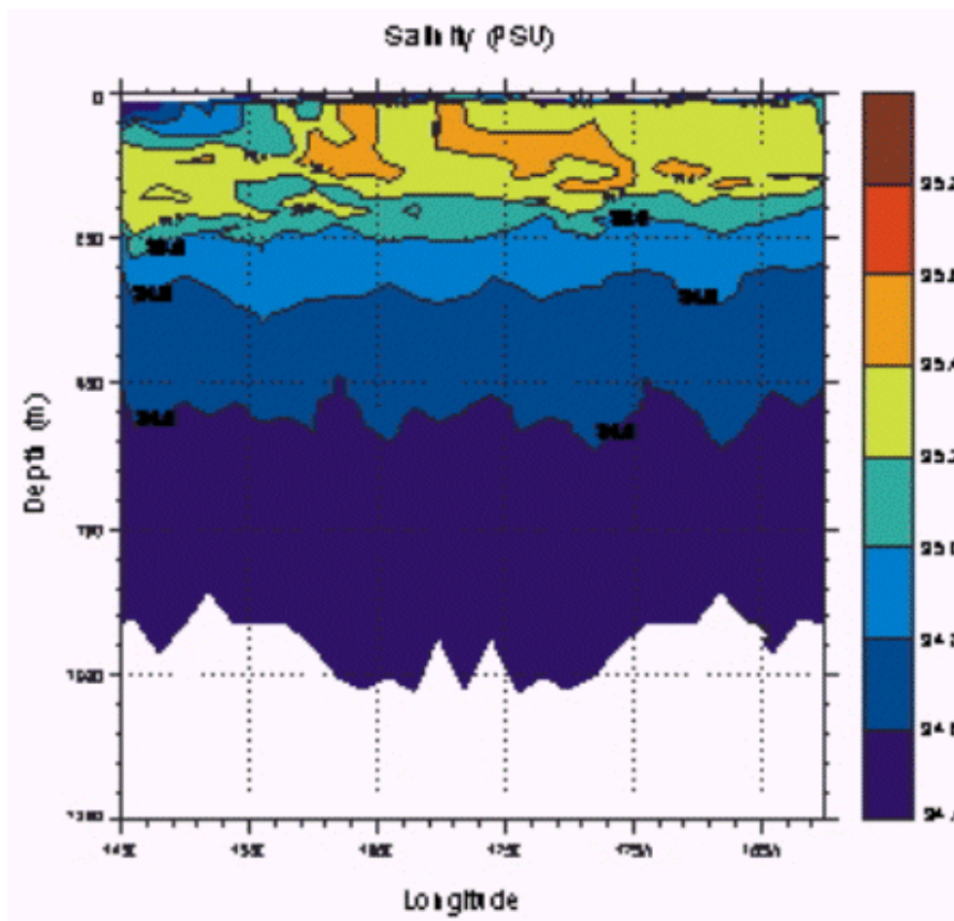
Fig.3 Vertical Section of Salinity (by XCTD)
