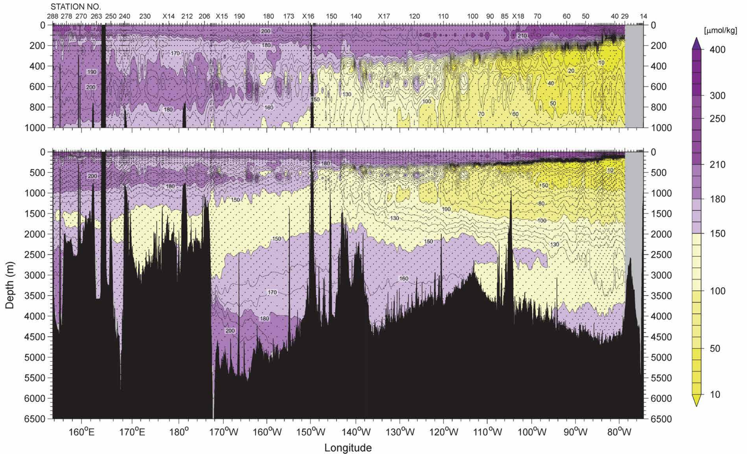
Figure 15 Bottle sampled dissolved oxygen ( \mu\text{mol/kg} )
