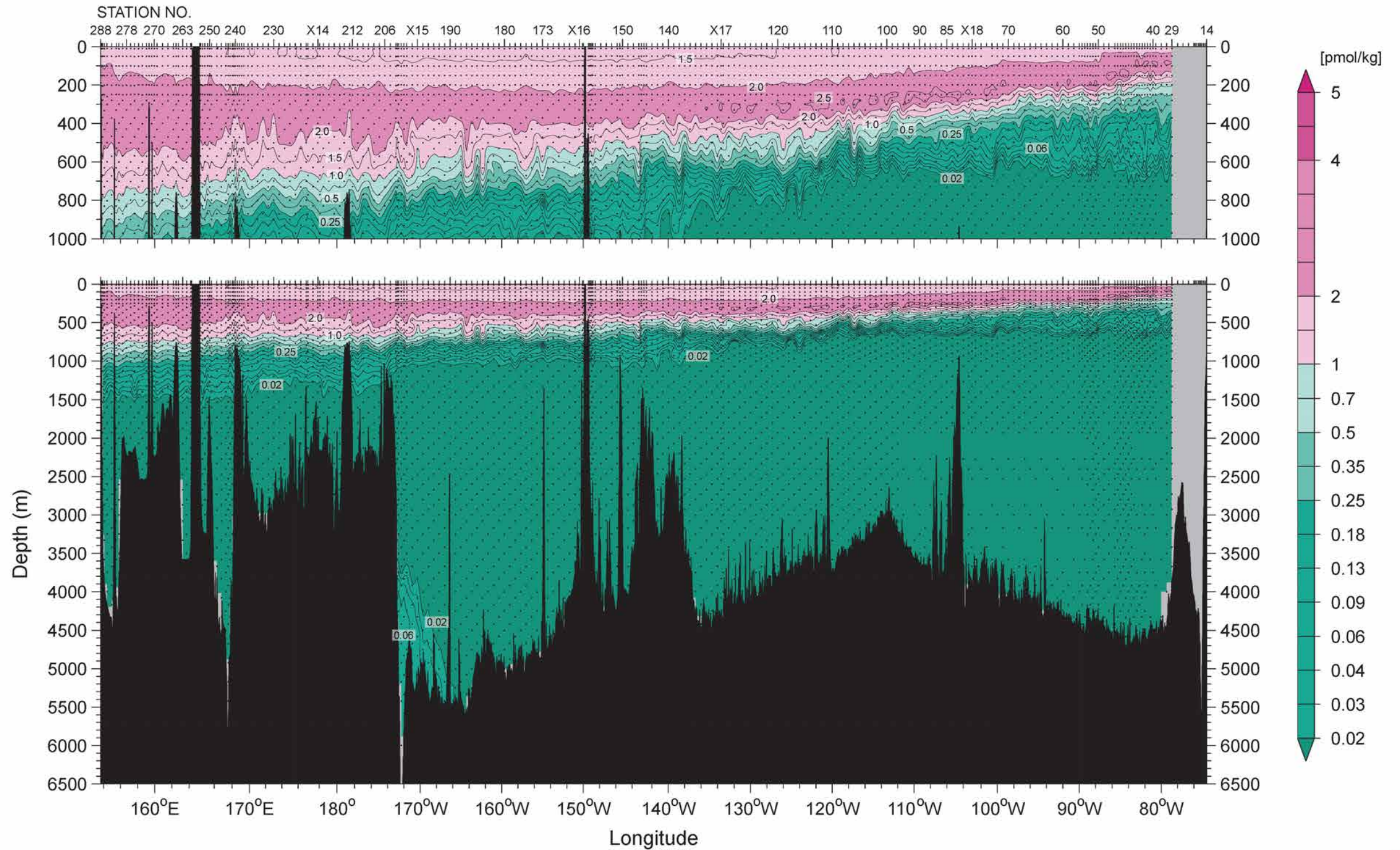
Figure 23 CFC-11 (pmol/kg)
