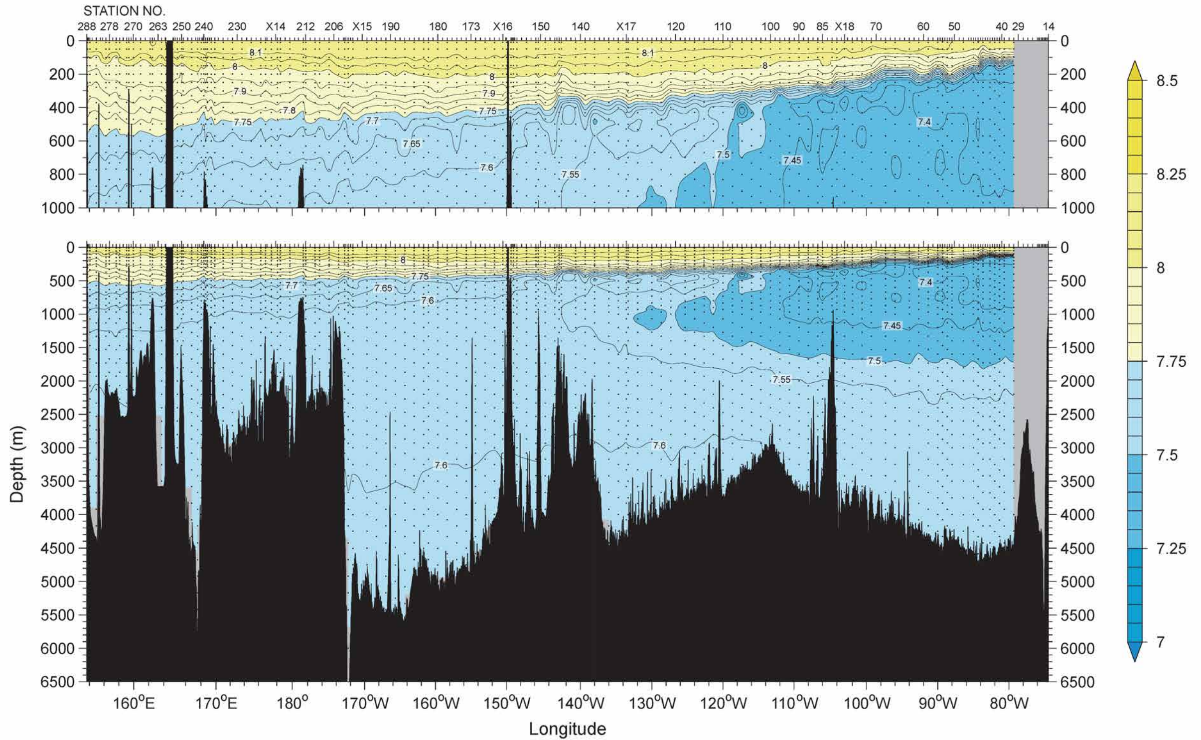
Figure 22 pH (pH T )
