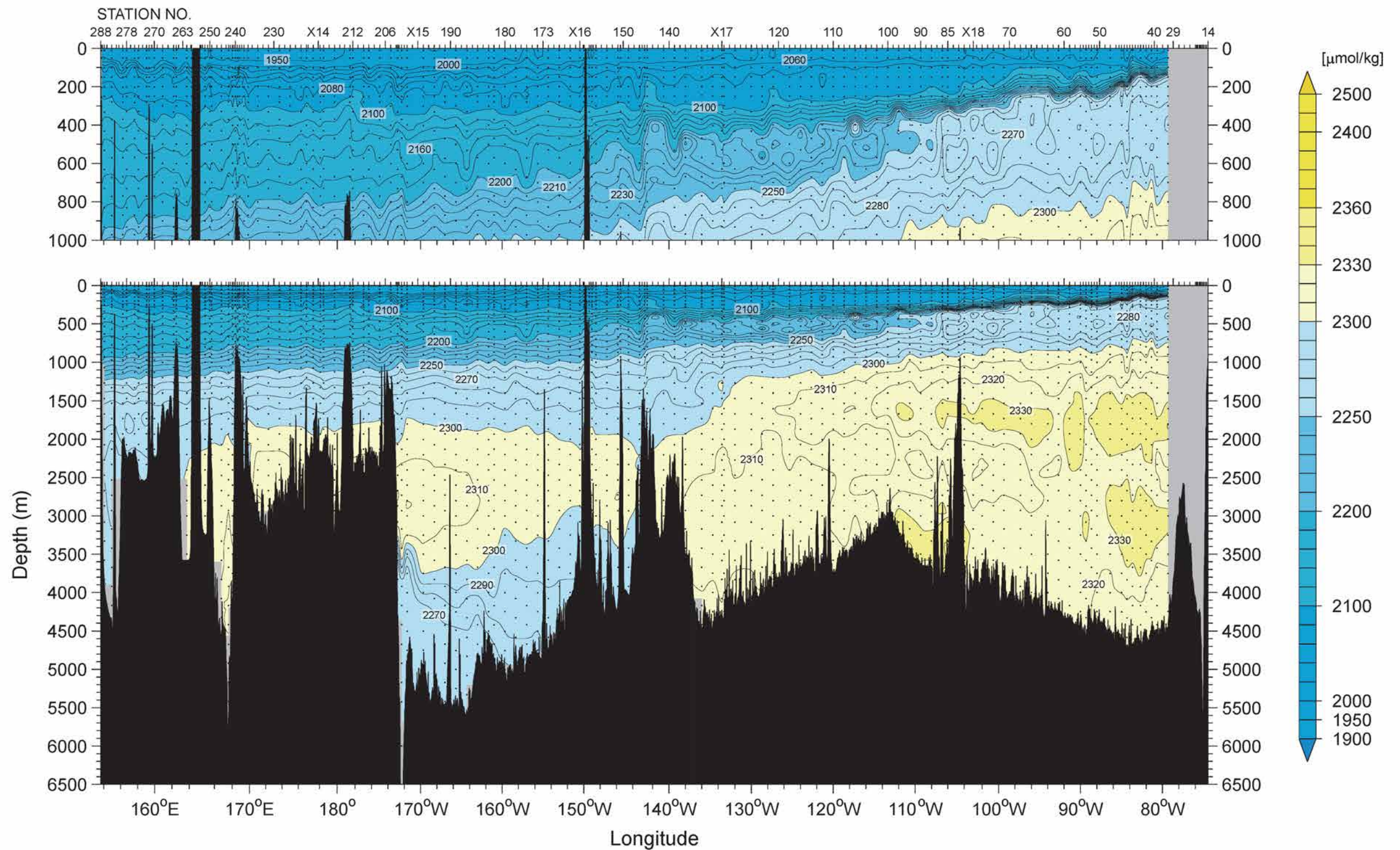
Figure 20 Dissolved inorganic carbon ( C_T ) ( \mu\text{mol/kg} )
