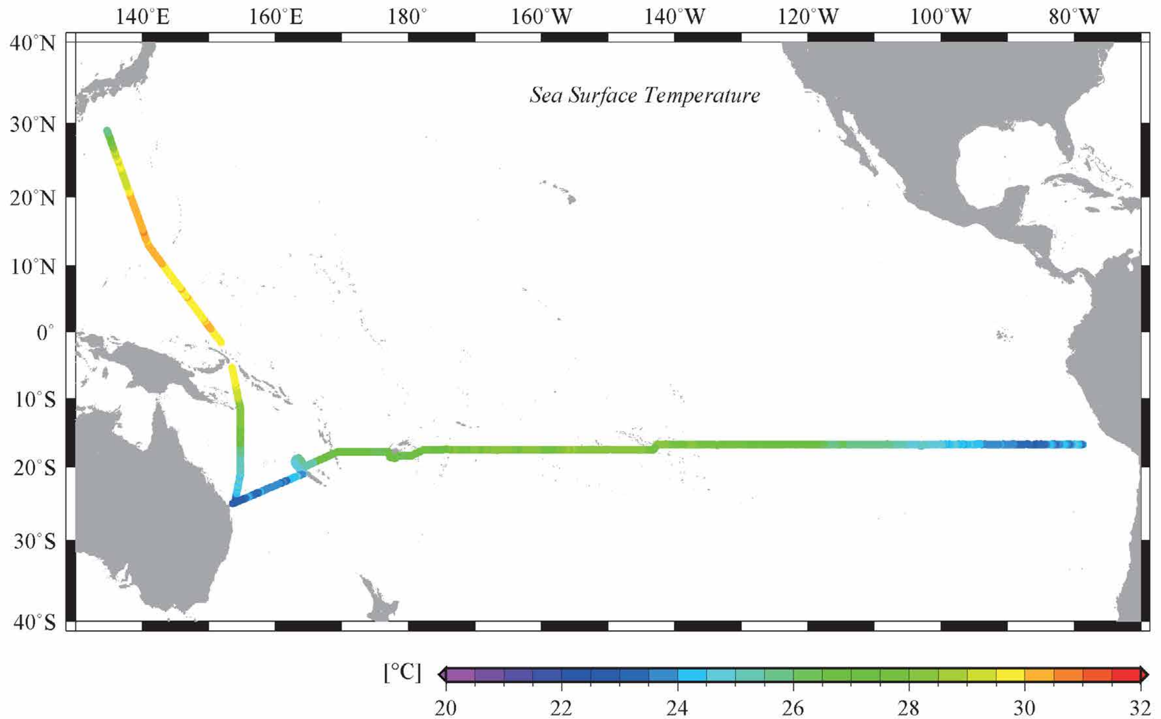
Figure 4 Sea surface temperature (SST)
