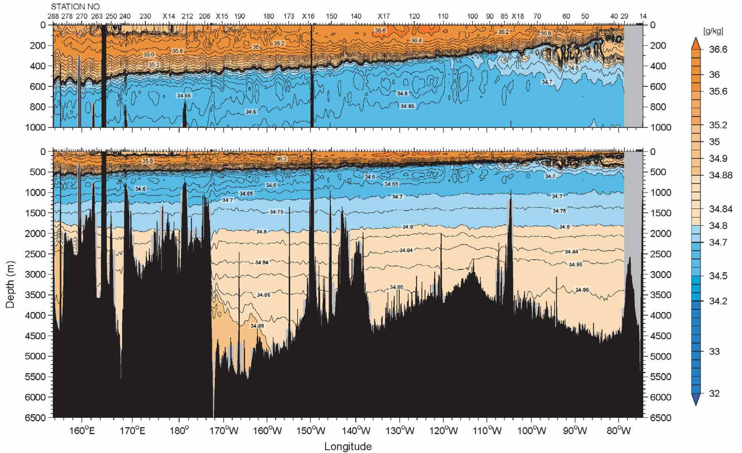
Figure 10 Absolute salinity (g/kg)
