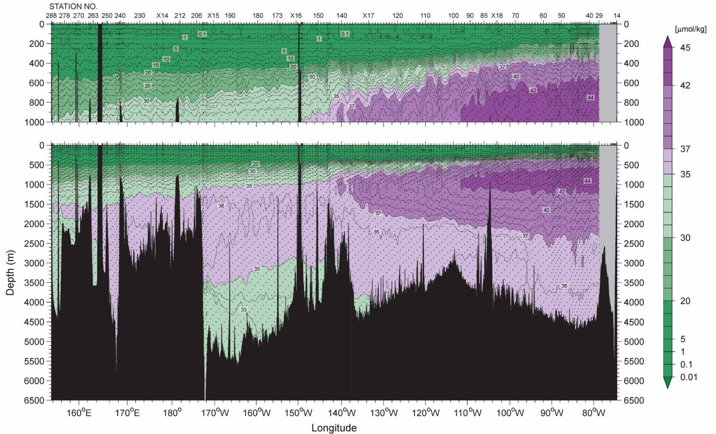
Figure 17 Nitrate ( \mu\text{mol/kg} )
