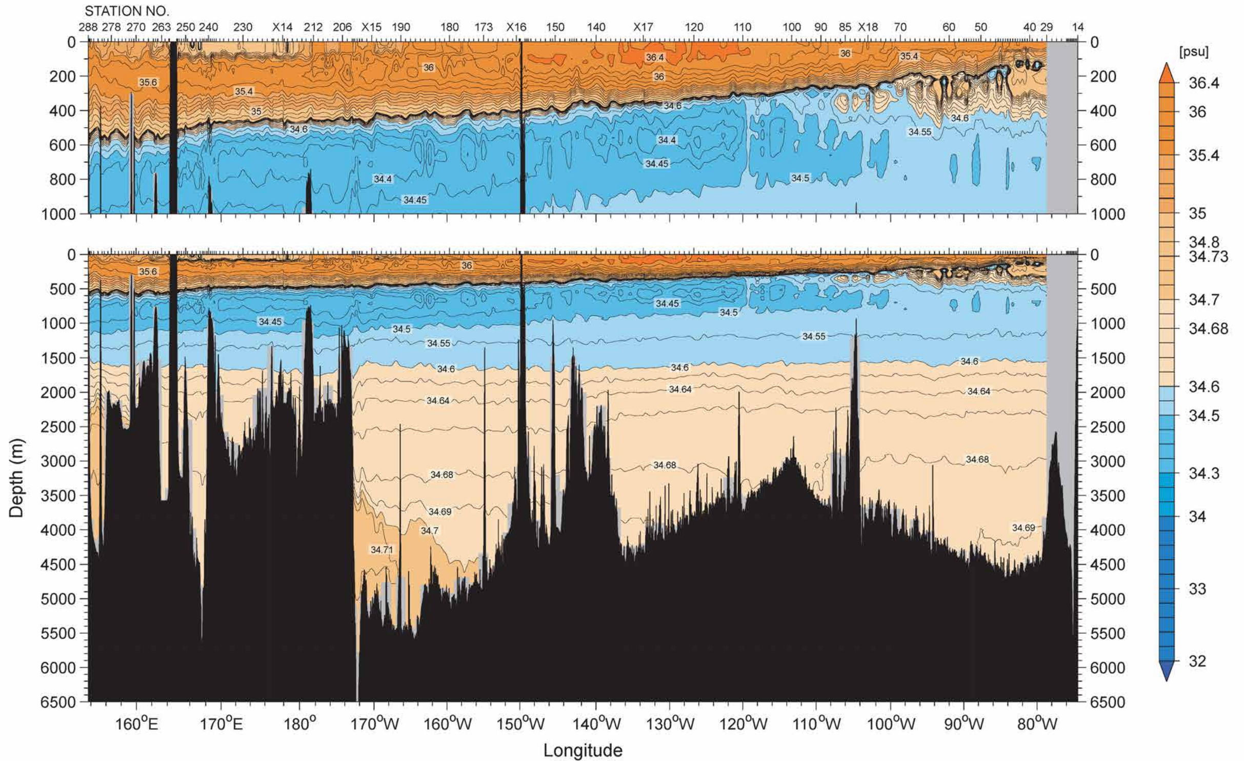
Figure 9 CTD salinity (psu)
