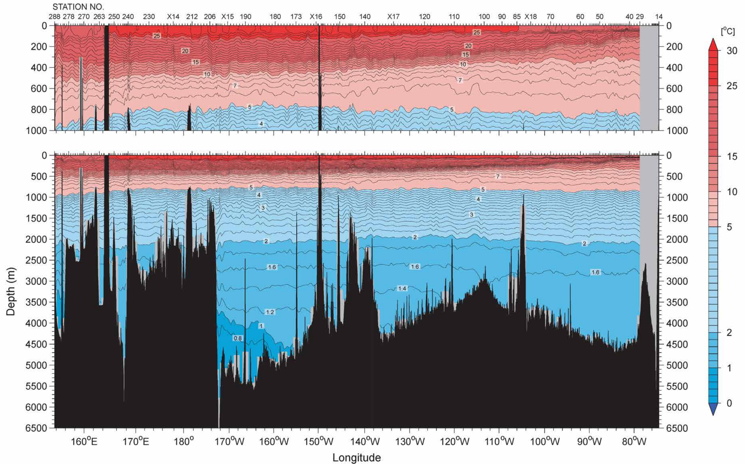
Figure 8 Potential temperature (°C)
