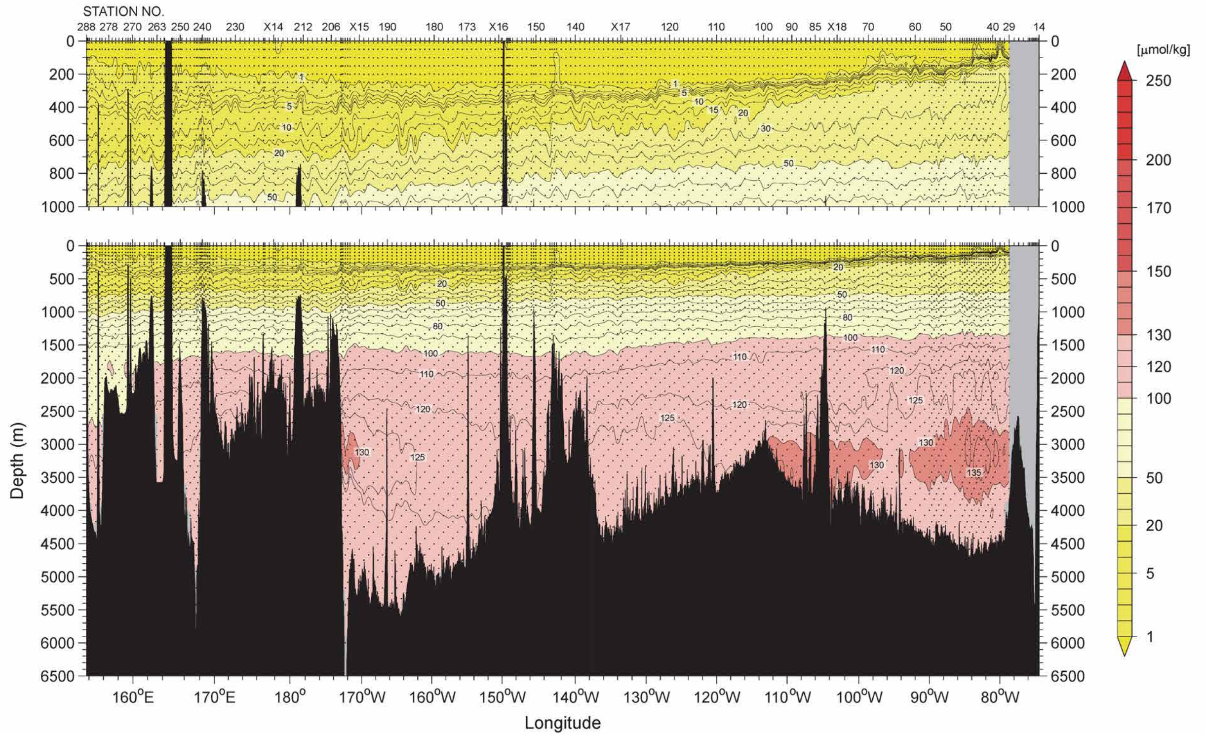
Figure 16 Silicate ( \mu\text{mol/kg} )
