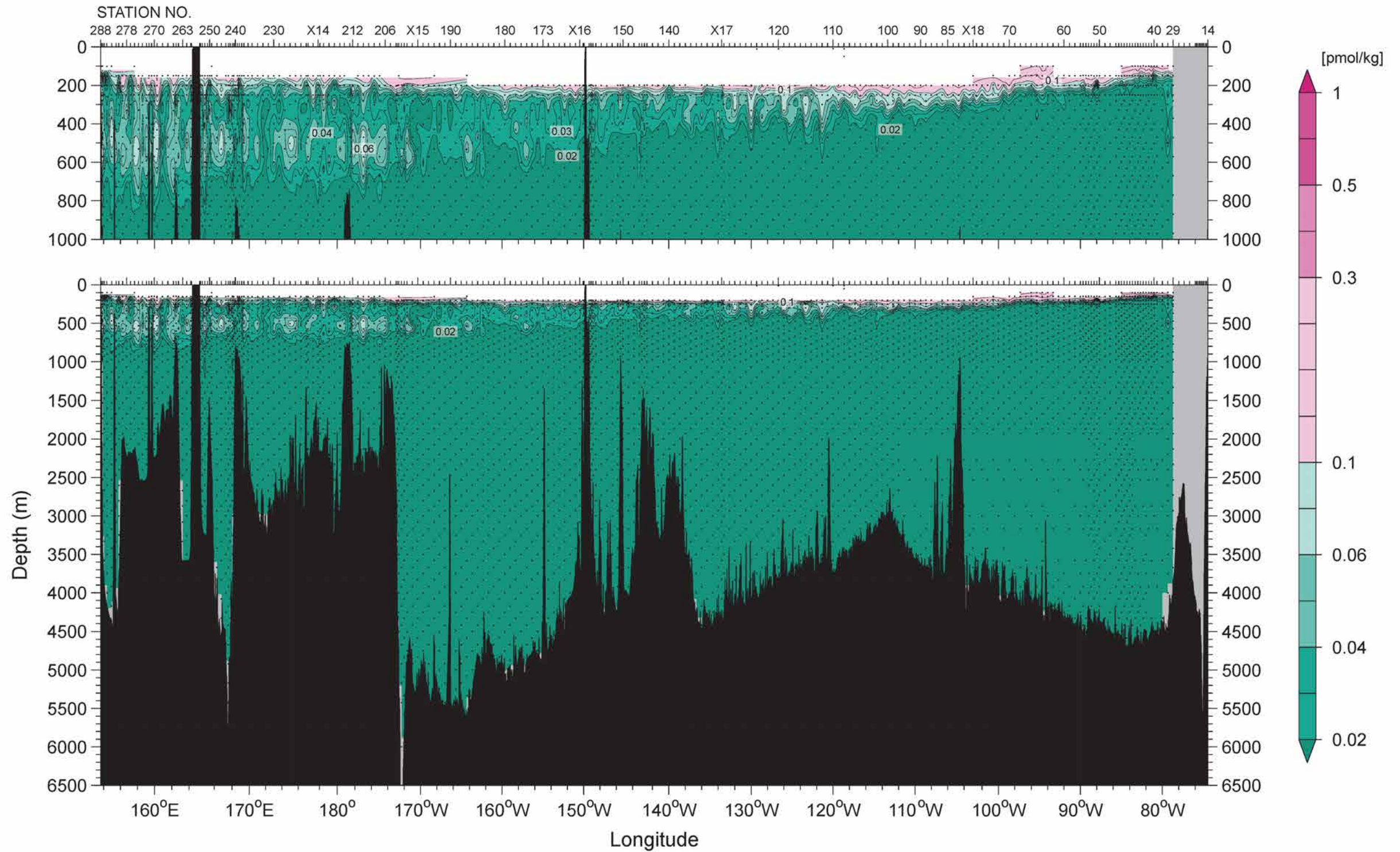
Figure 25 CFC-113 (pmol/kg)
