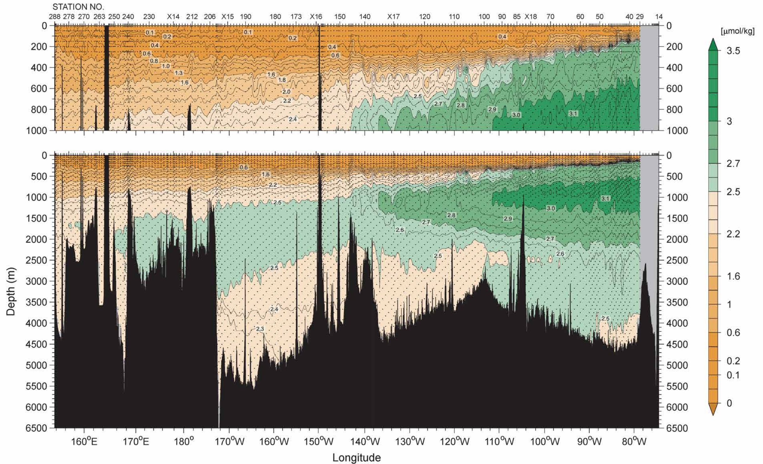
Figure 19 Phosphate ( \mu\text{mol}/\text{kg} )
