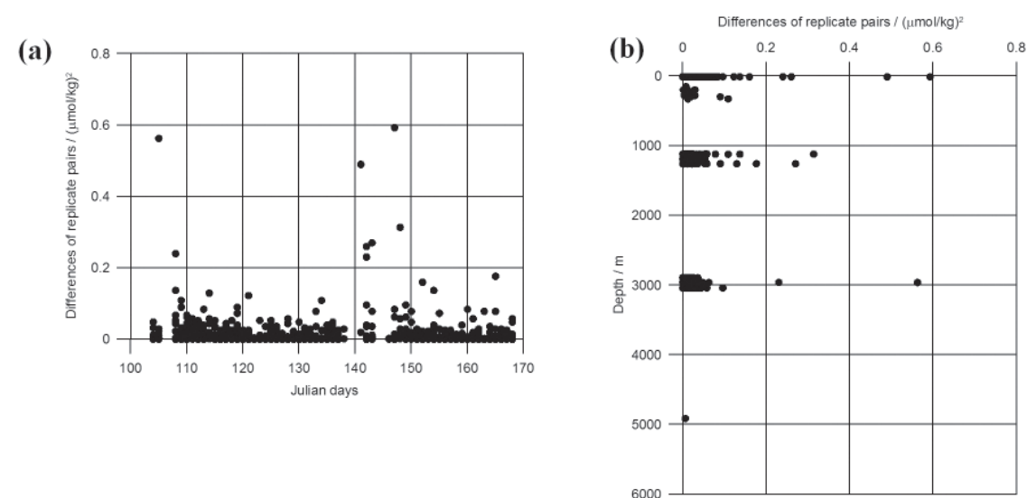
Figure 3.3.1. Differences ( (\mu\text{mol kg}^{-1})^2 ) of replicate sample pairs against the Julian days (a) and sampling depth (b).
