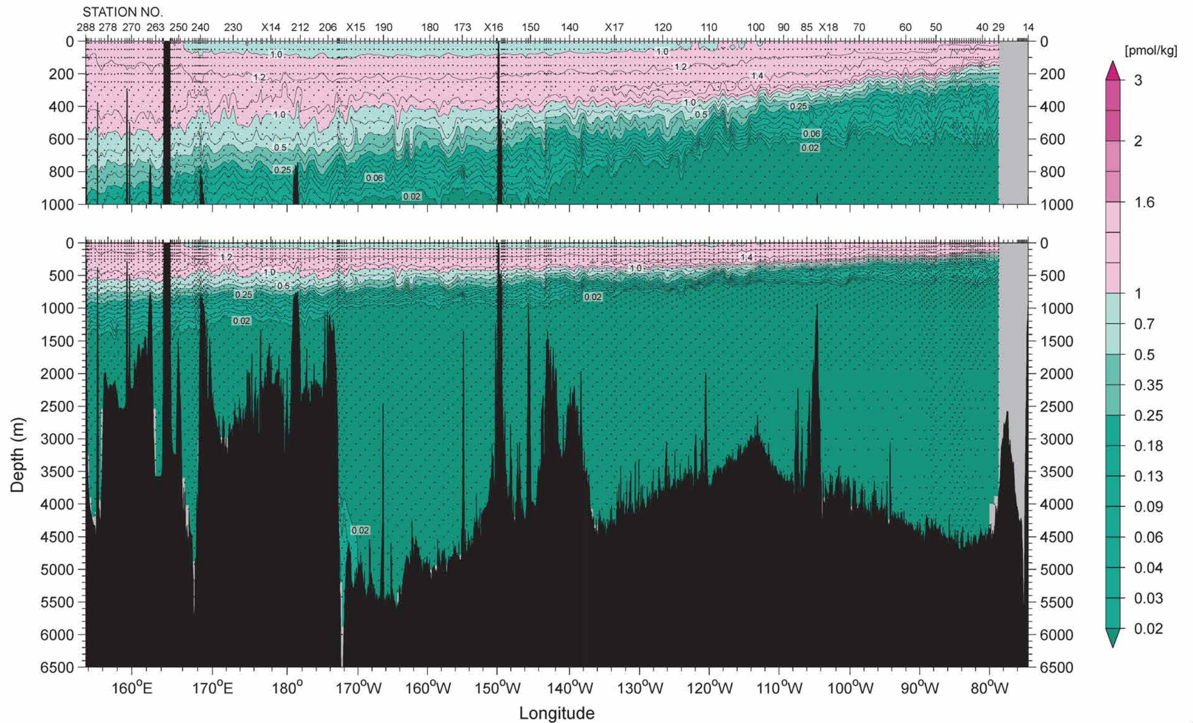
Figure 24 CFC-12 (pmol/kg)
