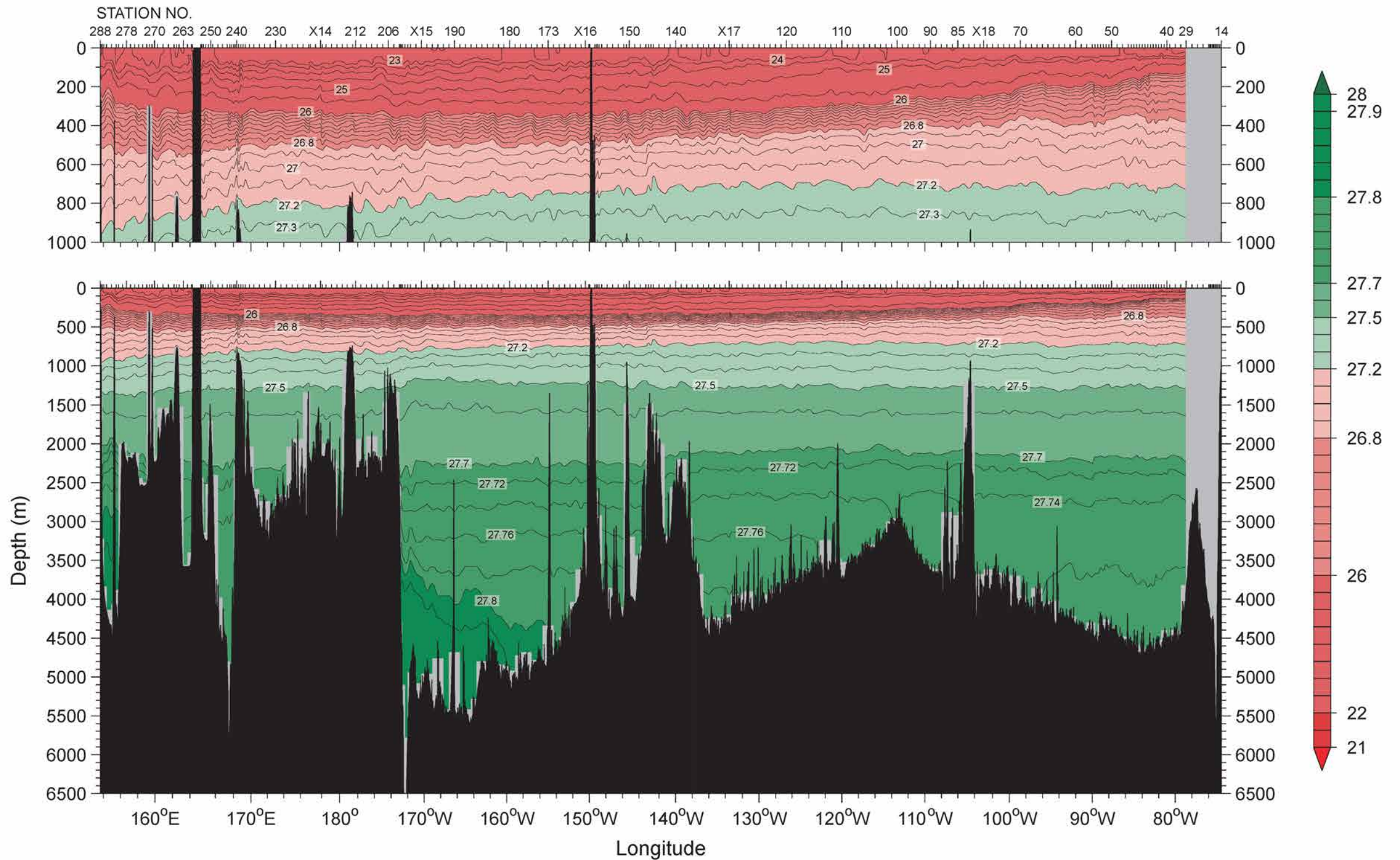
Figure 11 Density ( \sigma_0 ) ( \text{kg/m}^3 )
