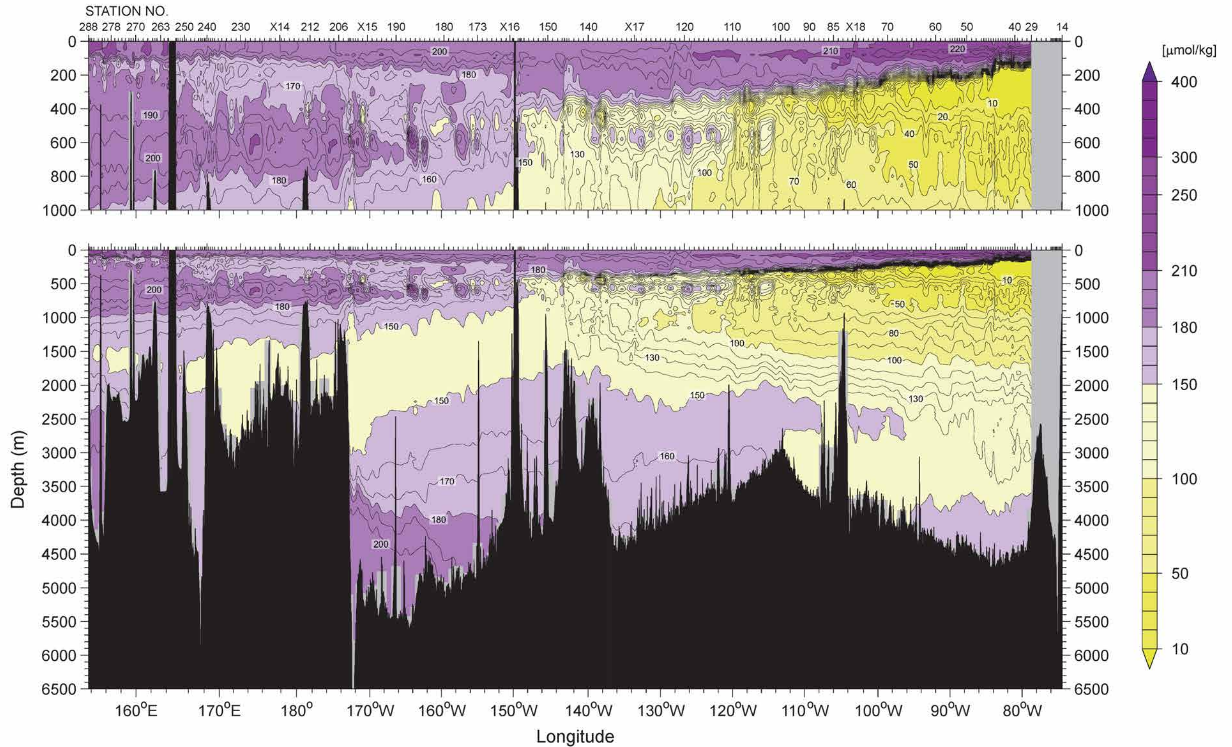
Figure 14 CTD oxygen ( \mu\text{mol/kg} )
