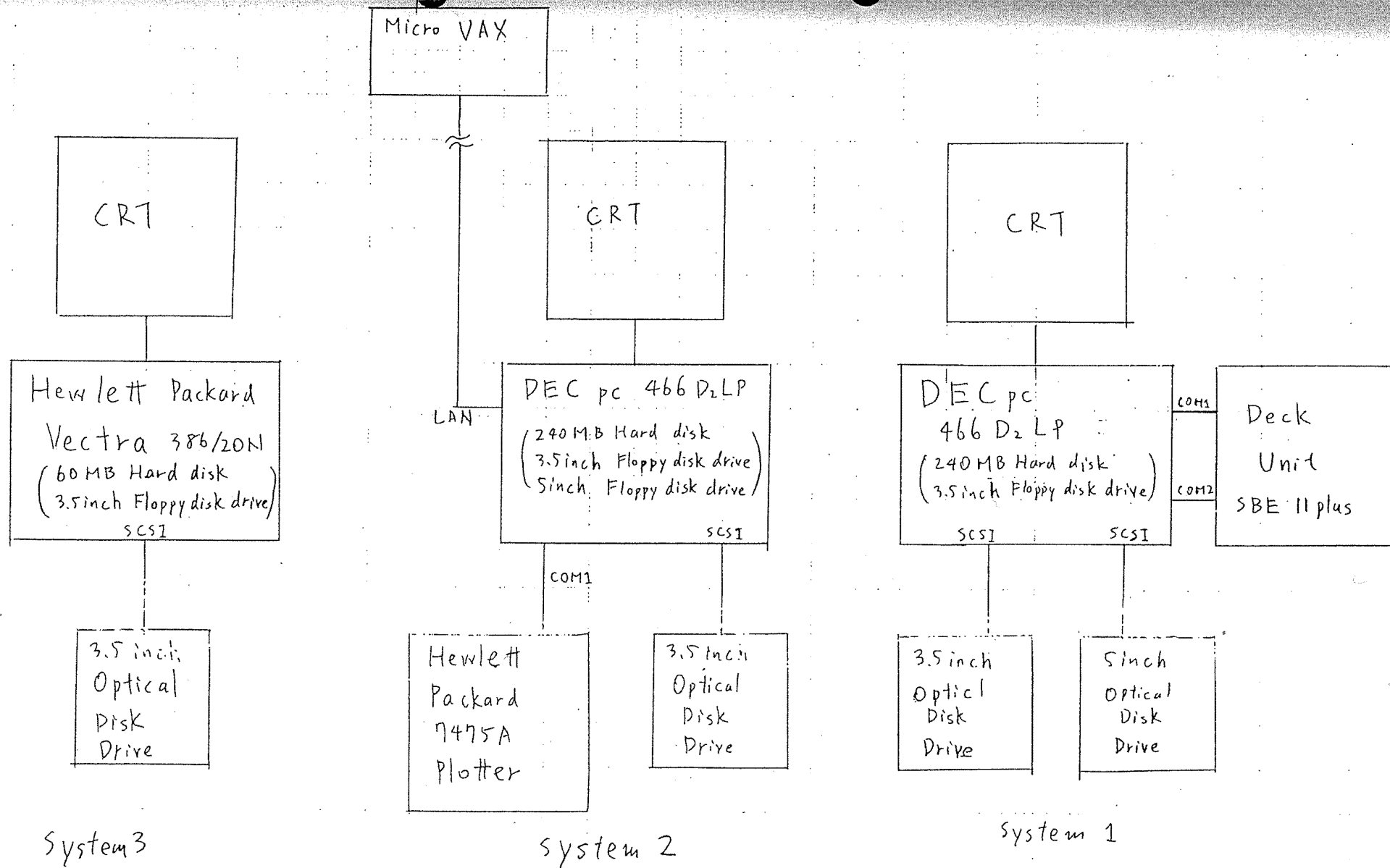
Figure 11-1 Computer systems for CTD data processing
