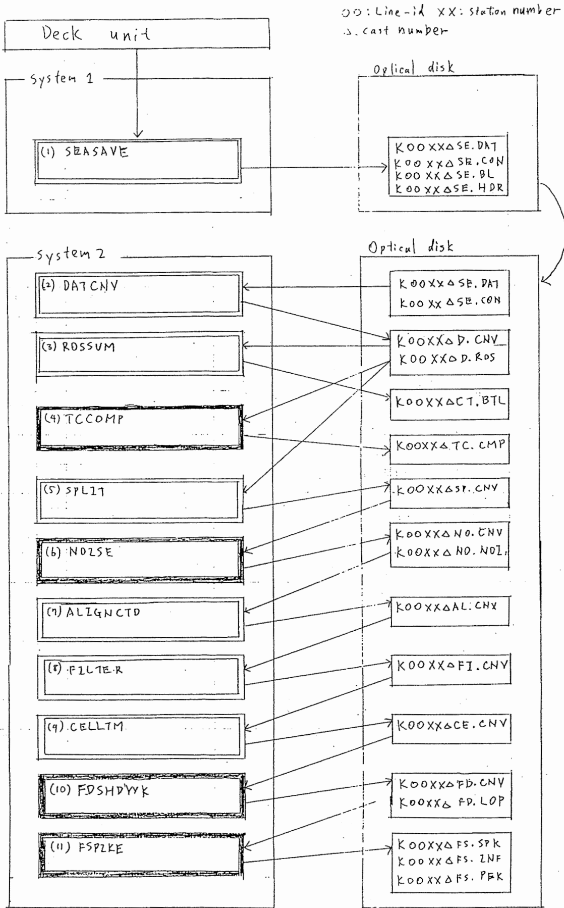
Figure 11-6 Data flow of CTD data processing
