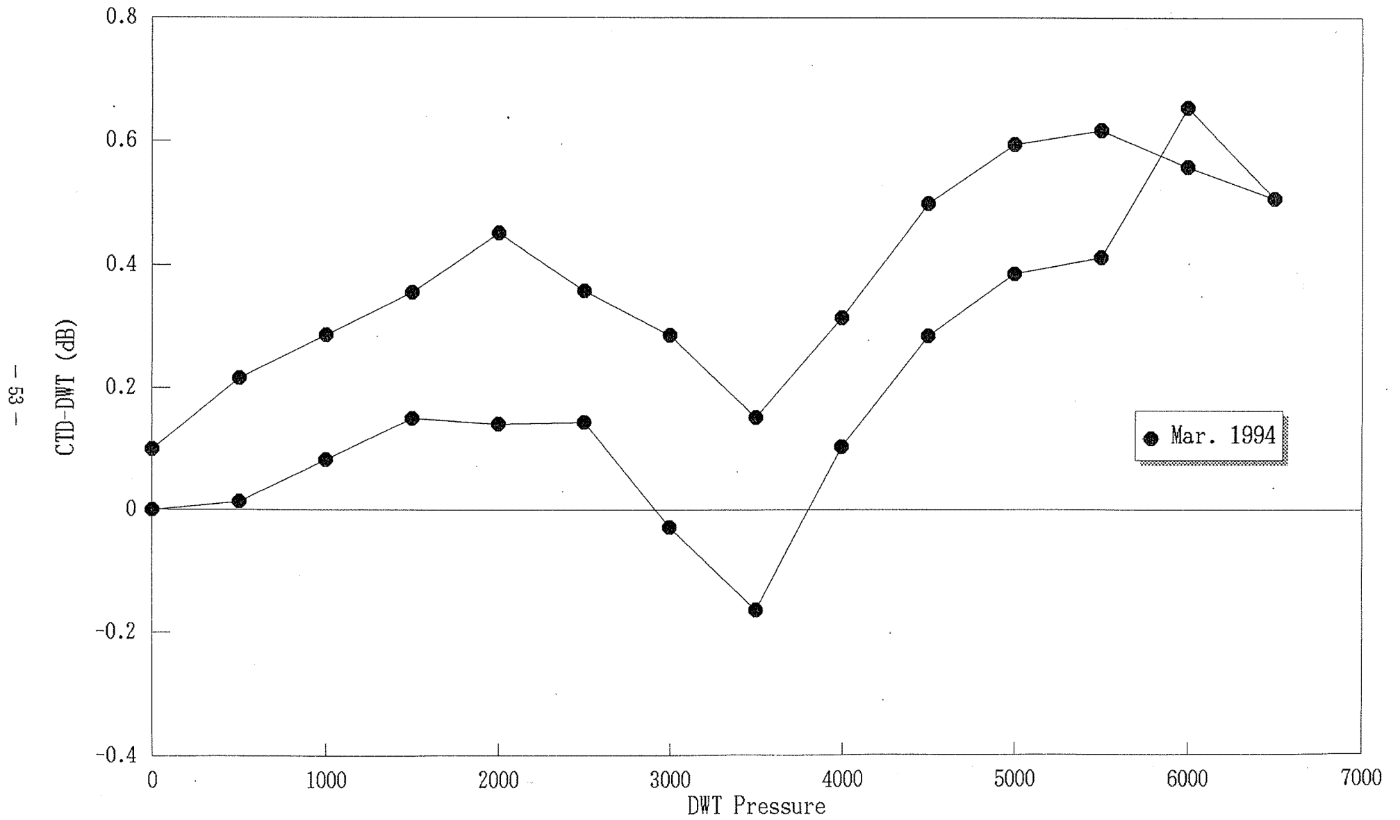
Fig.11-5 Calibration of Pressure Sensor
