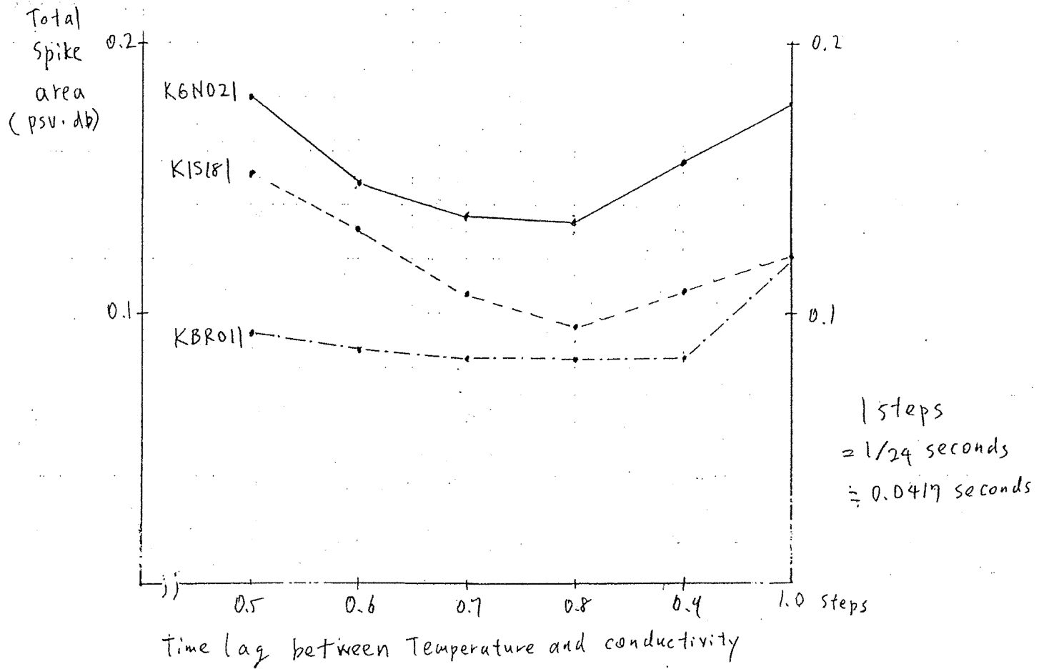
Figure 11-2 Total salinity spike area variability for time lag between Temperature and conductivity at casts K6N021, K15181 and KBRO11
