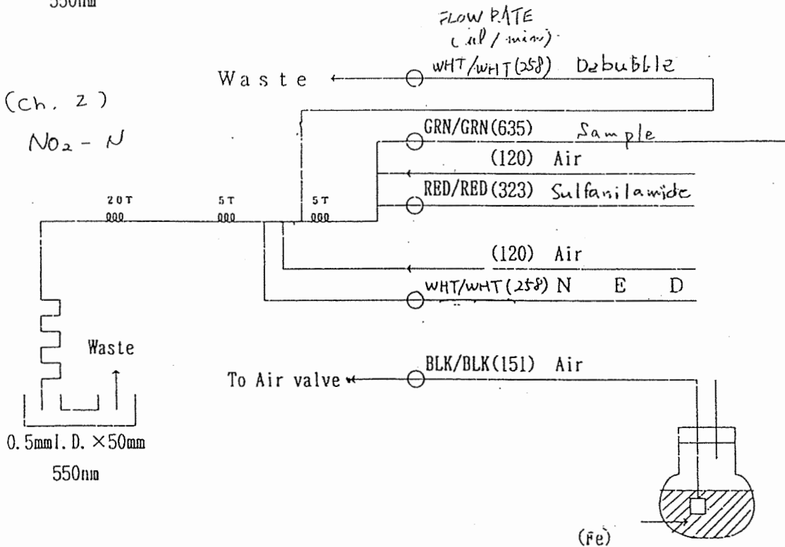
Figure 14-1 (upper) Flow diagram for TRAACS 800 nitrate method
