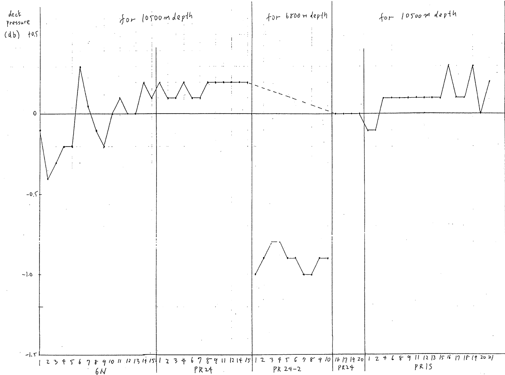
Figure 11-4 Variability of deck pressure
