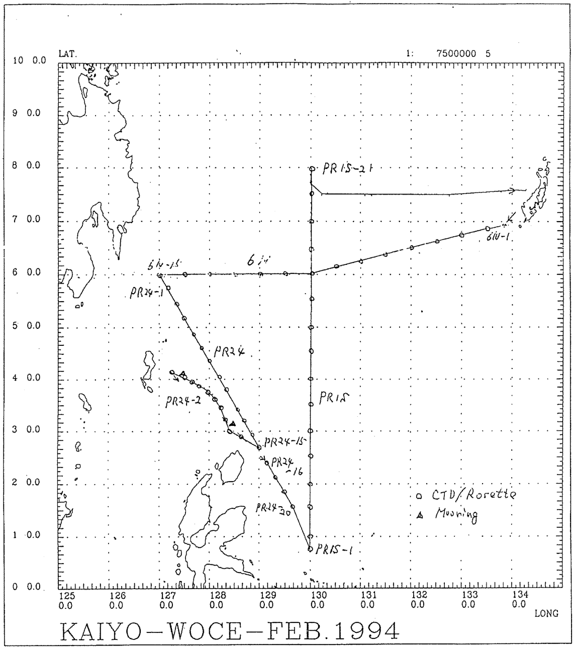
Figure 2-1 Track chart.
