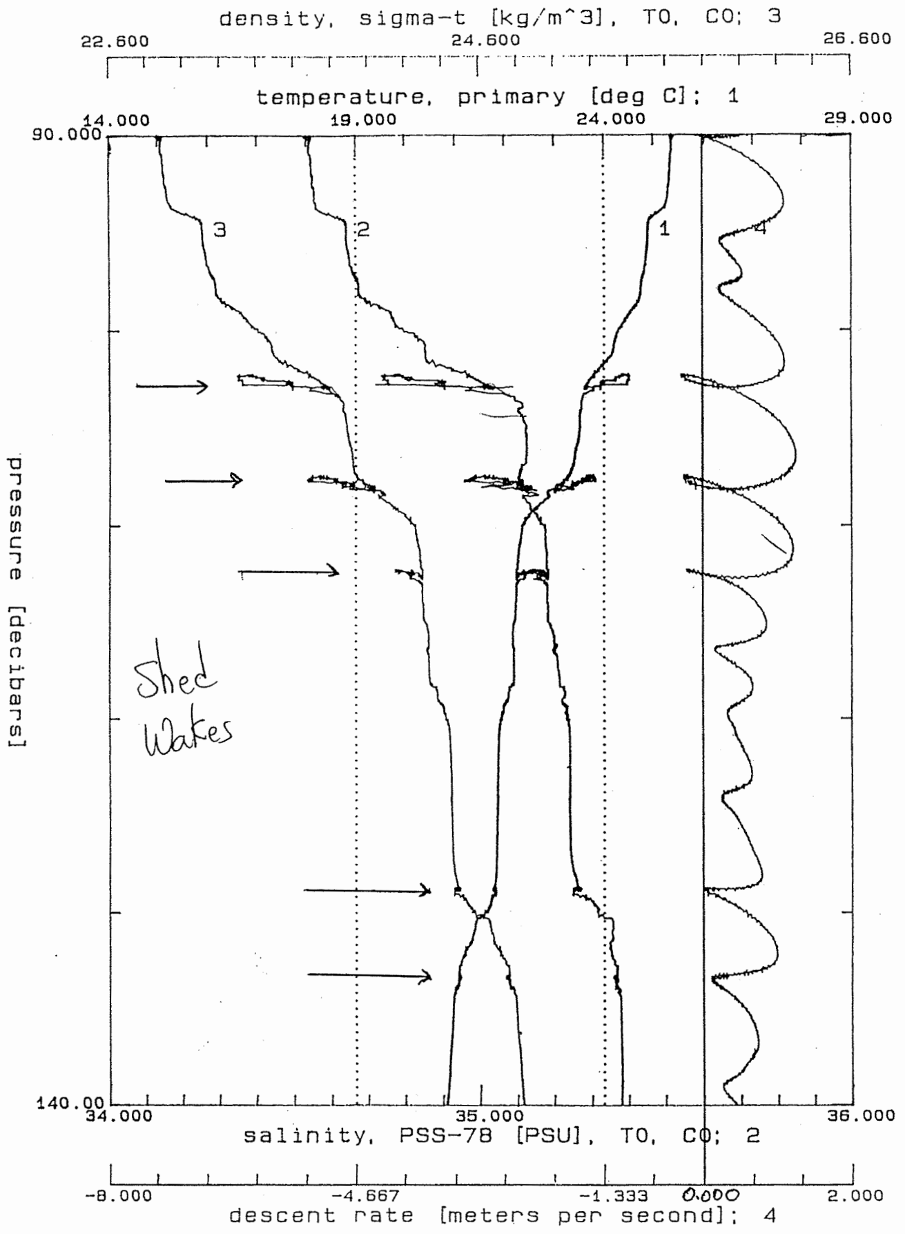
Figure 21-5 CAST K24201
