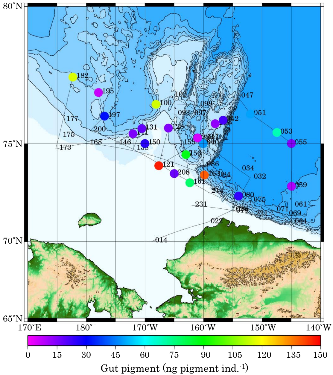
Fig. 3-11-4. Geographical distribution of gut pigment of Calanus hyperboreus C6F.
