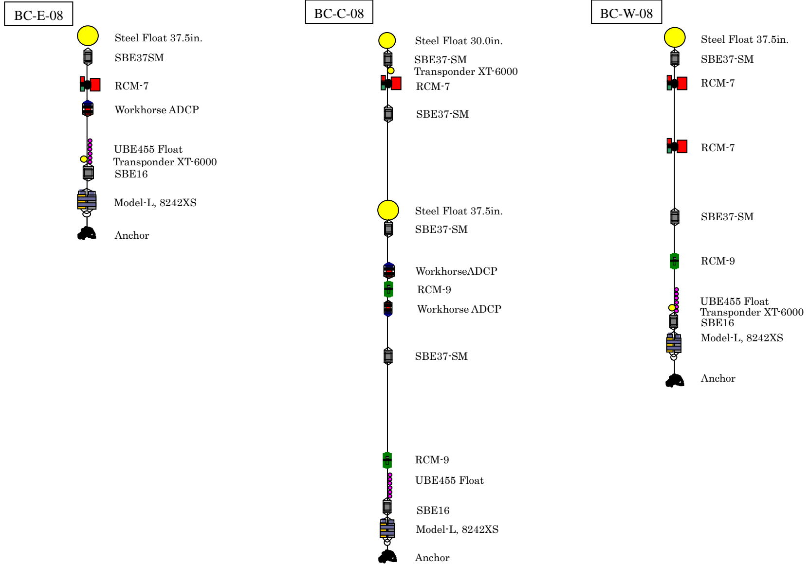
Fig.2-4-2 Mooring diagram of Deployment moorings
