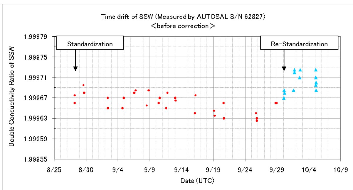
Fig. 2.2-1 History of double conductivity ratio for the Standard Seawater batch P149
