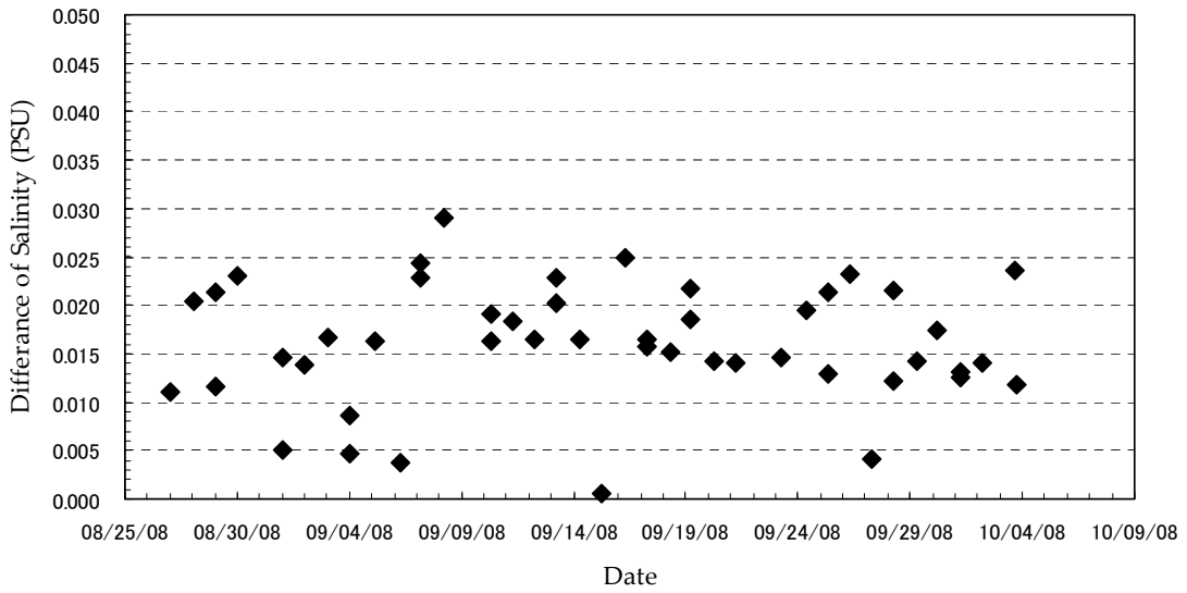
Fig.2.5-3 Difference of salinity between sensor data and bottle data. The mean difference is 0.0161psu.
