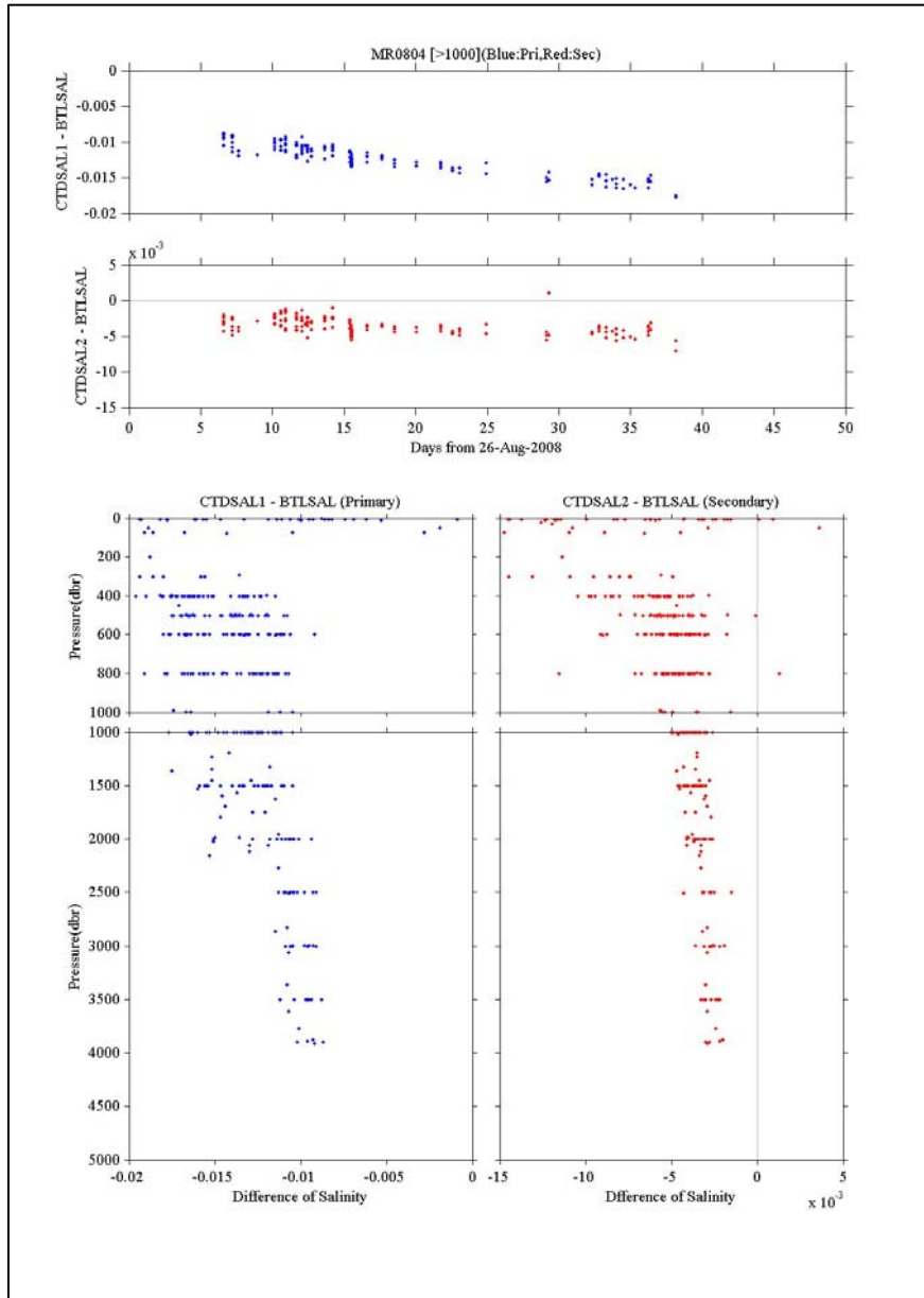
Fig 2.1-2 Time drift and the difference between CTD salinity and BTL salinity
