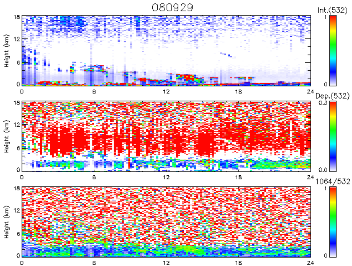
Fig 4.8.-1. Lidar data on Sept.29, 2008, during MR08-04.
