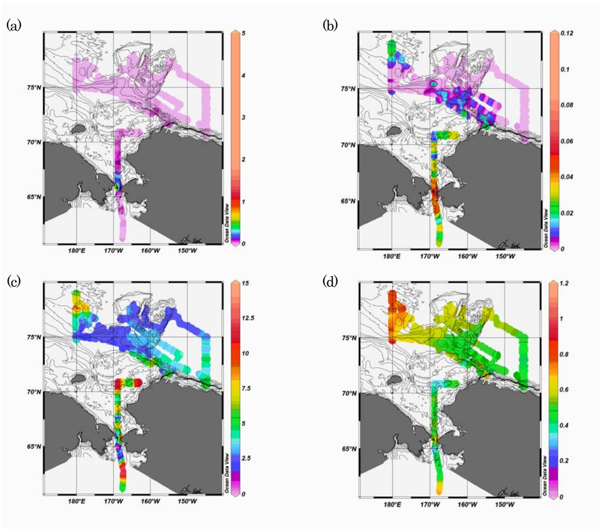
Figure 3.2-1-1. Profile of Sea surface nutrients. (a) Nitrate + Nitrite, (b) Nitrite, (c) Silicate and (d) Phosphate (unit: \mu\text{M} ). Period of observation: 27-Aug. -2008 23:53 to 3-Oct -2008 06:21 (UTC).
