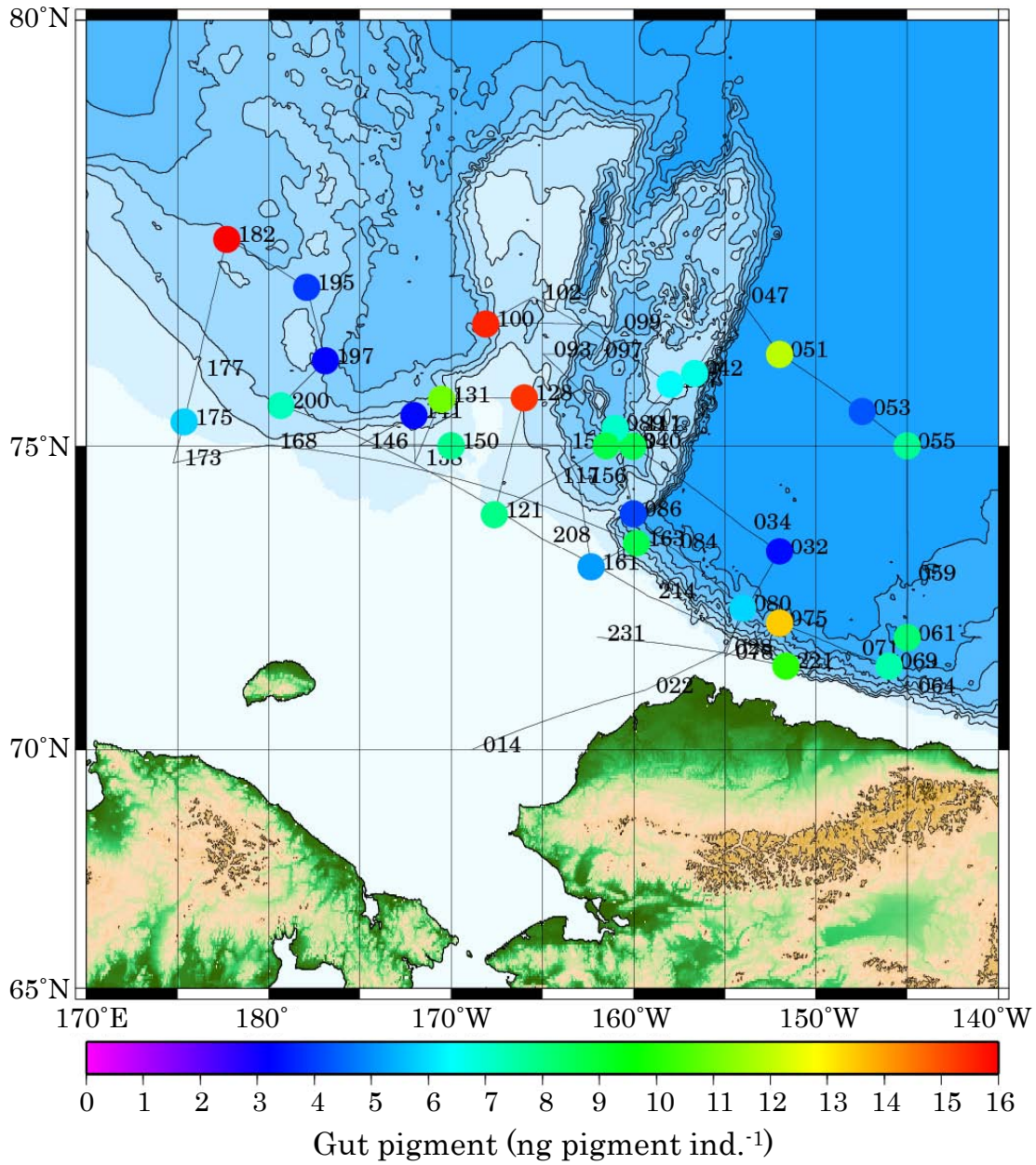
Fig. 3-11-5. Geographical distribution of gut pigment of Metridia longa C6F.
