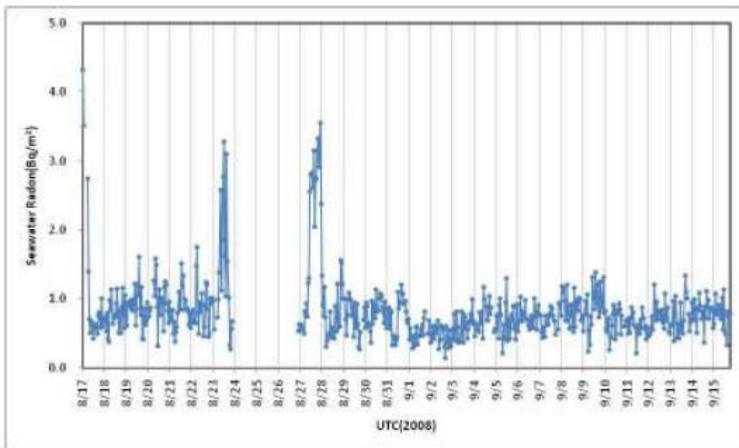
Fig.3.12-3 Seawater Radon Concentration in Cruise MR08-04 from August-17 to September-15, 2008.
