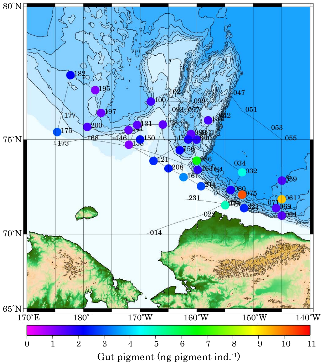
Fig. 3-11-2. Geographical distribution of gut pigment of Calanus glacialis C5.
