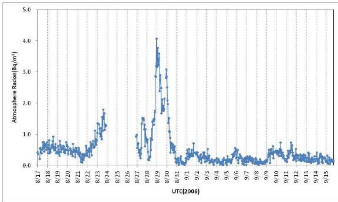
Fig.3.12-1 Atmospheric Radon Concentration in Cruise MR08-04 from August-17 to September-15, 2008.
