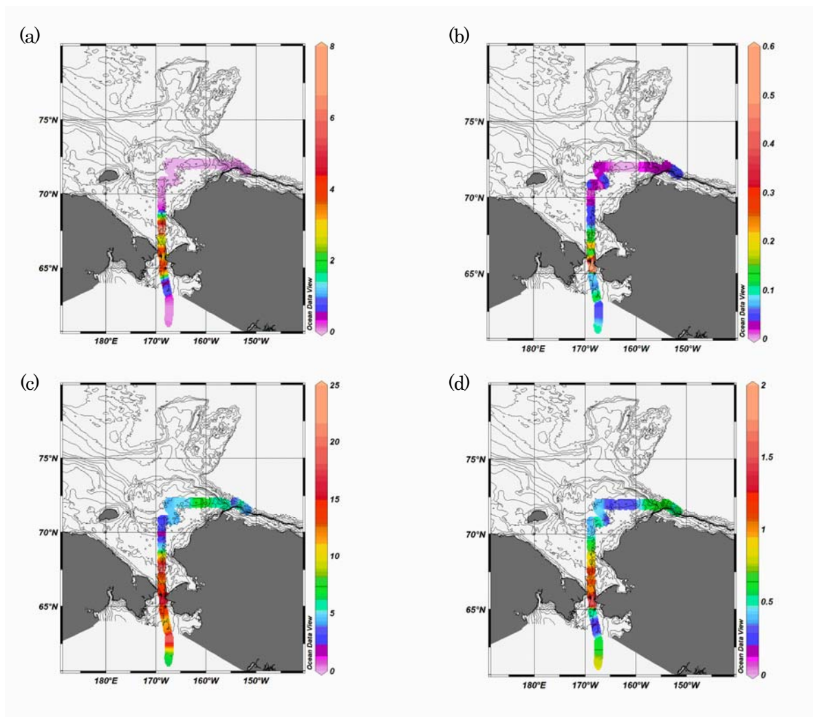
Figure 3.2-1-2. Profile of Sea surface nutrients. (a) Nitrate + Nitrite, (b) Nitrite, (c) Silicate and (d) Phosphate (unit: \mu\text{M} ). Period of observation: 3 -Oct. -2008 08:10 to 7-Oct -2008 15:52 (UTC).
