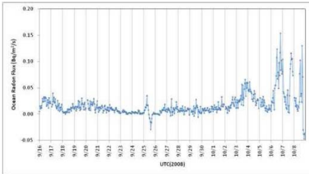
Fig.3.12-6 Ocean Radon Flux in Cruise MR08-04 from September-16 to October-8, 2007.
