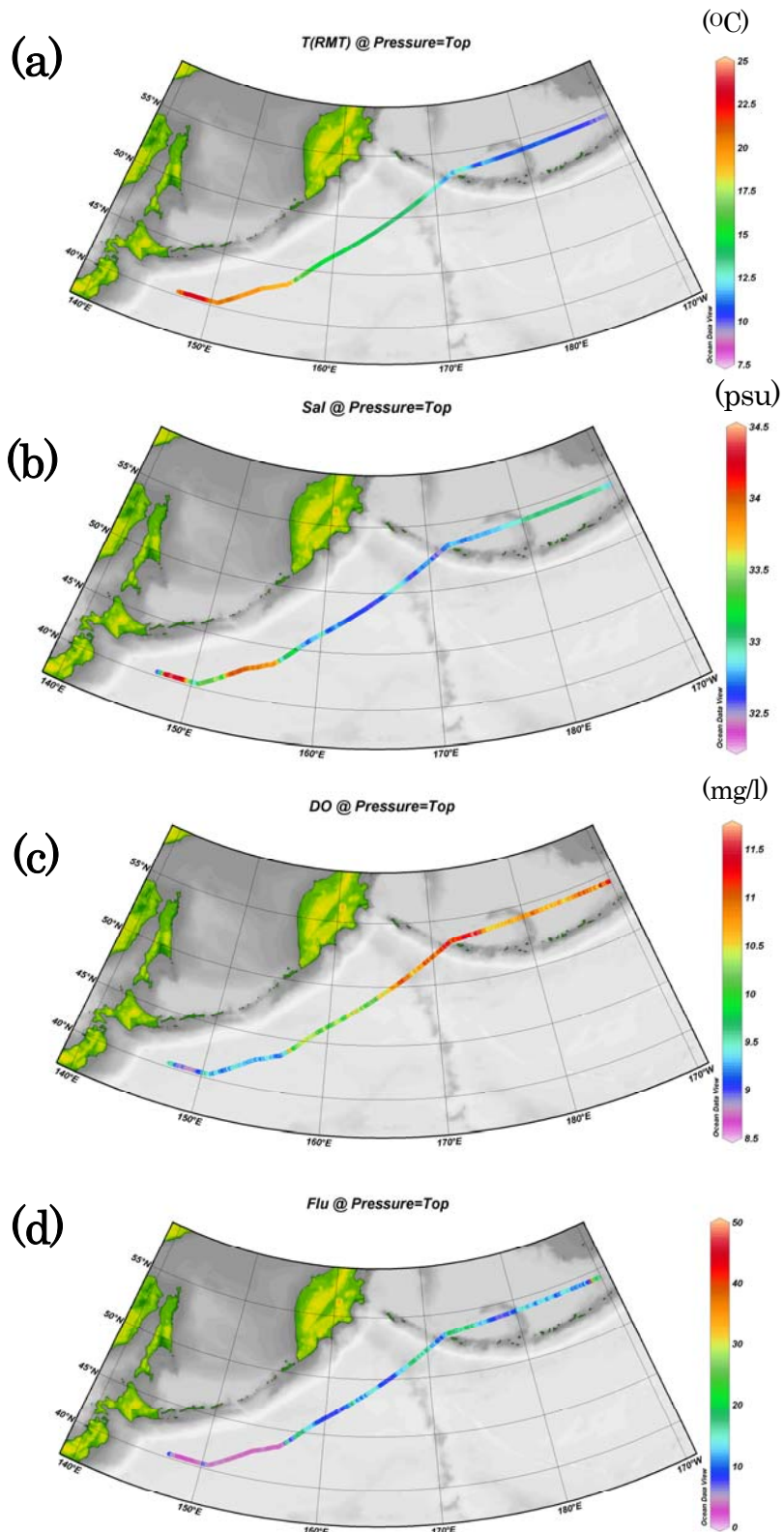
Fig.2.5-1 Spatial and temporal distribution of (a) temperature, (b) salinity, (c) dissolved oxygen and (d) fluorescence in MR08-04 LEG1 cruise. Fluorescence is relative value.
