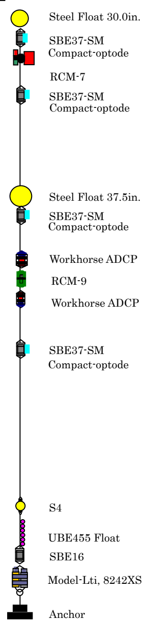
Fig.2-4-1a Mooring diagram of Recovery moorings
