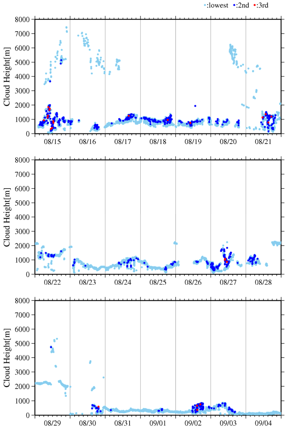
Fig.4.5-1 Lowest, 2nd and 3rd cloud base height during the cruise.
