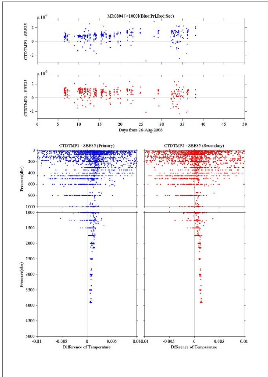
Fig 2.1-1 Time drift and the difference between CTD temperature and SBE35
