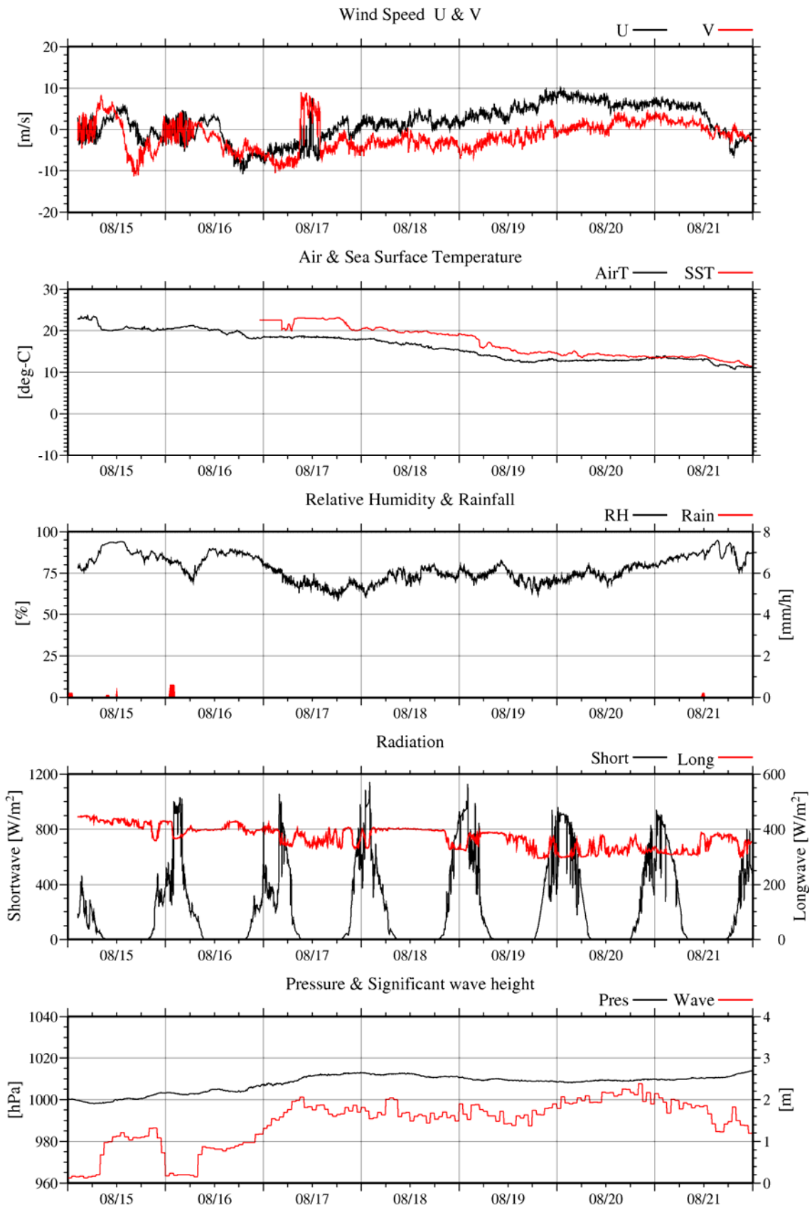
Fig.4.4-1 Time series of surface meteorological parameters during the MR08-04 cruise
