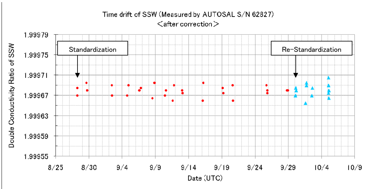
Fig. 2.2-2 History of double conductivity ratio for the Standard Seawater batch P149 (S/N 62827: after correction)
