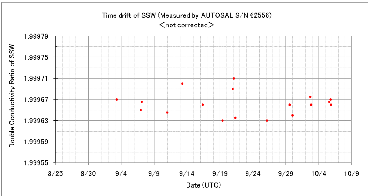
Fig. 2.2-3 History of double conductivity ratio for the Standard Seawater batch P149 (S/N 62556: not corrected)
