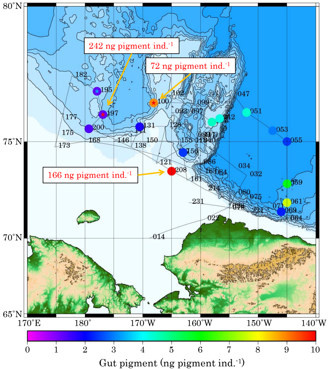
Fig. 3-11-3. Geographical distribution of gut pigment of Calanus glacialis C6F. Stars denote gut pigment for parasite (dinoflagellate Ellobiopsis sp.) attached individual.
