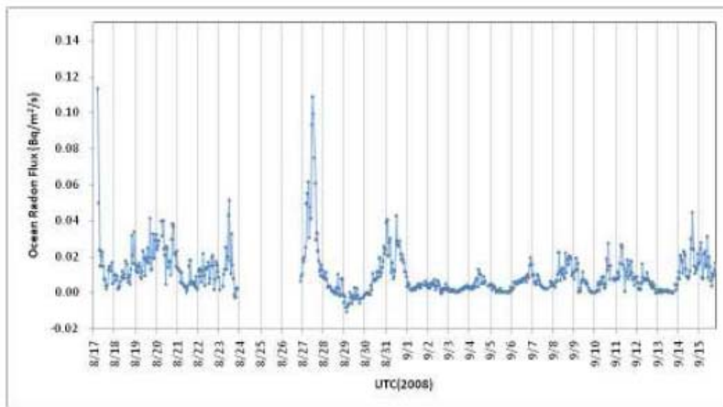
Fig.3.12-5 Ocean Radon Flux in Cruise MR08-04 from August-17 to Sempther-15, 2007.
