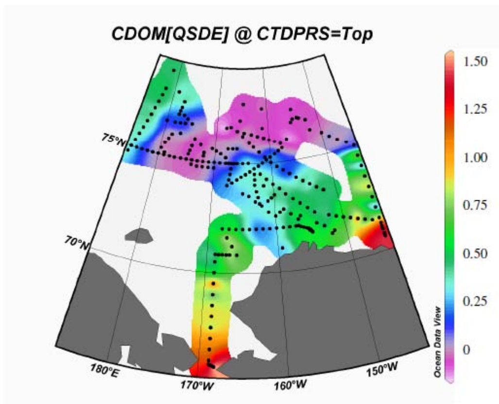
Fig. 1: Spatial variation of C-DOM concentrations at depth 5m. A post-calibration of CDOM concentration is currently underway.
