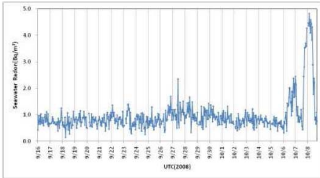
Fig.3.12-4 Seawater Radon Concentration in Cruise MR08-04 from September-16 to October-8, 2008.
