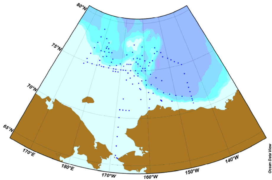
Fig. 3.8-1. Sampling stations for study area. Chl- a samples were collected at 132 stations.
