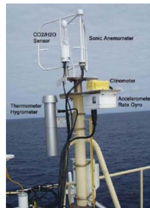
Fig. 4.9-1 Turbulent flux measurement system on the top deck of the foremast.
