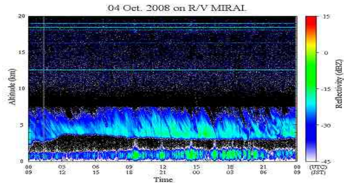
Fig 4.6.-2. Time height cross section of radar reflectivity factor in dBZe on Oct. 04, 2008 during MR08-04 cruise.
