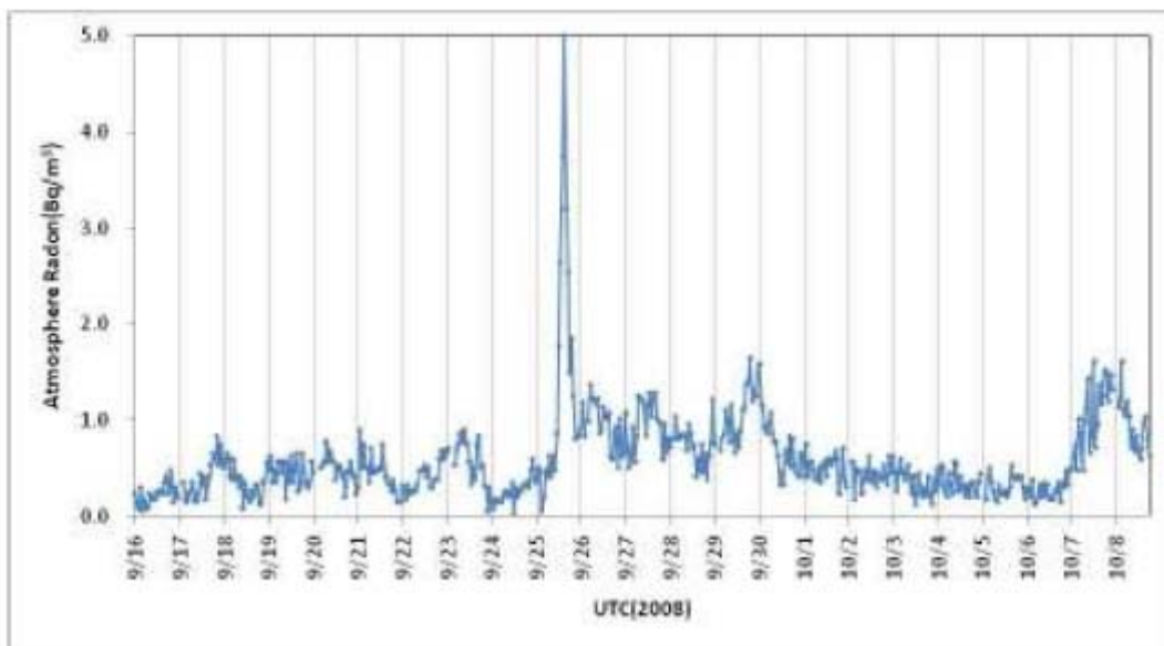
Fig.3.12-2 Atmospheric Radon Concentration in Cruise MR08-04 from September-16 to October-8, 2008.
