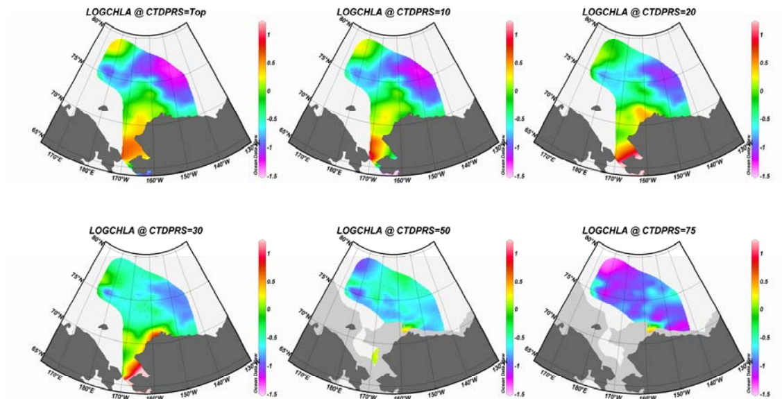
Fig. 3.8-2. Distribution of log-converted Chl- a concentrations for observed area at upper layer sampling depths (5, 10, 20, 30, 50 and 75 m).
