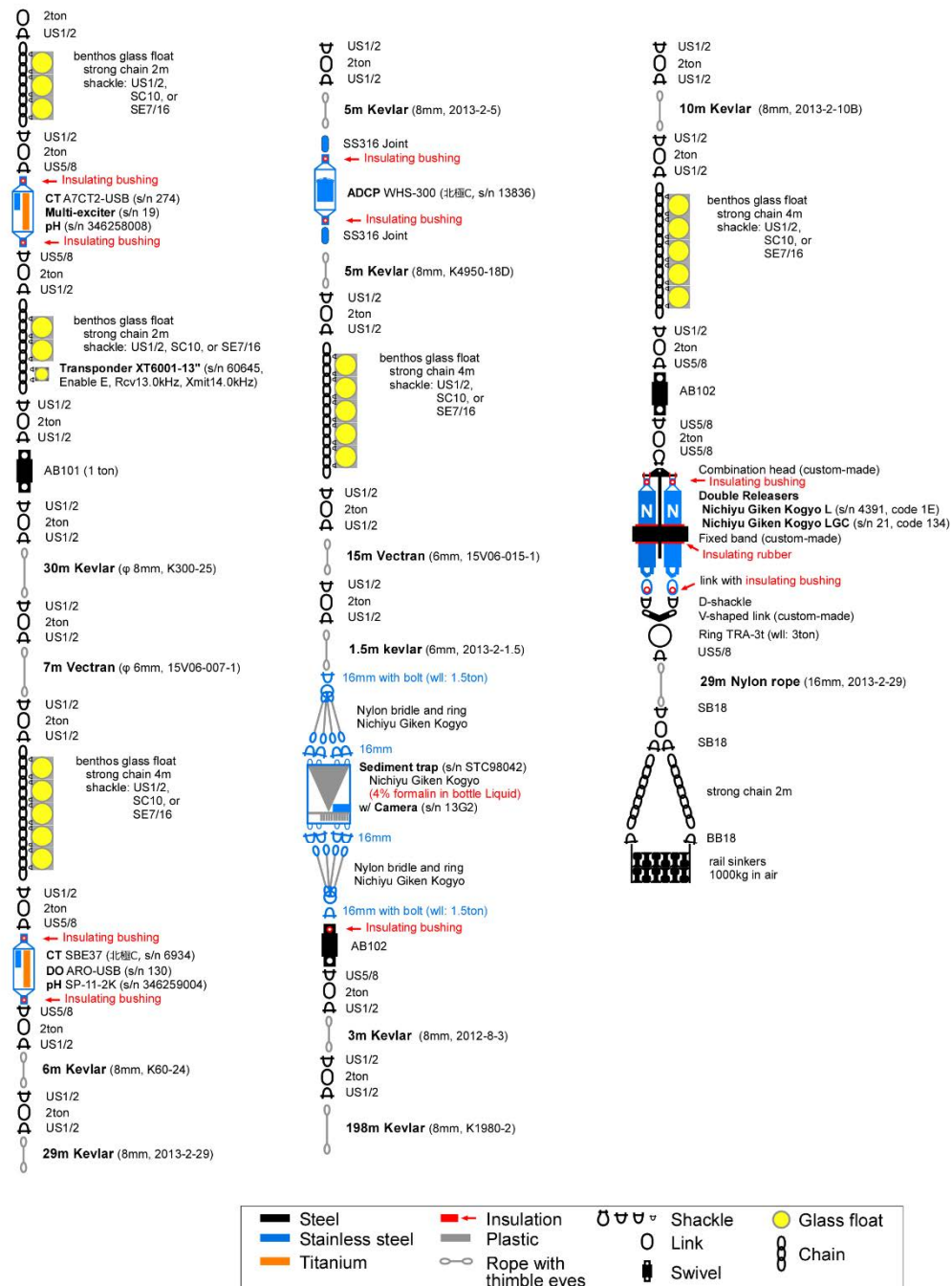
Fig. 4.21-5: The design of sediment trap mooring NHC15t.
