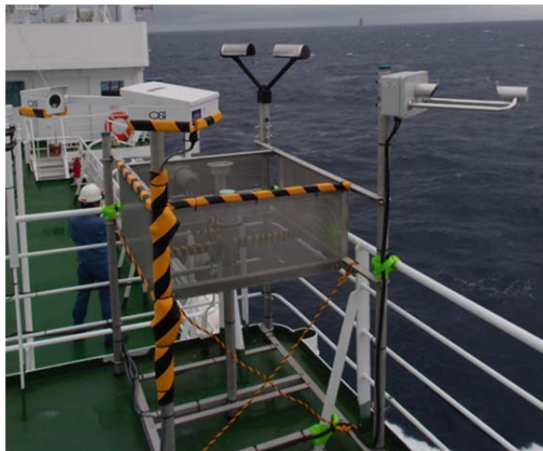
Fig. 2.4-1: The three disdrometers (Parsivel, LPM and Joss-Waldvogel disdrometer) and an optical rain gauge, installed on the roof of the anti-rolling tank.
