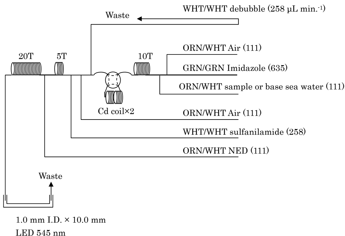
Figure 4.2-1 \text{NO}_3+\text{NO}_2 (1ch.) Flow diagram.
