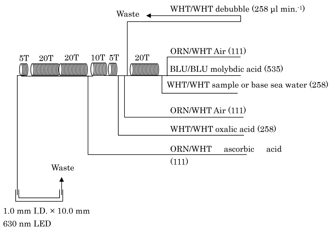
Figure 4.2-3 \text{SiO}_2 (3ch.) Flow diagram.
