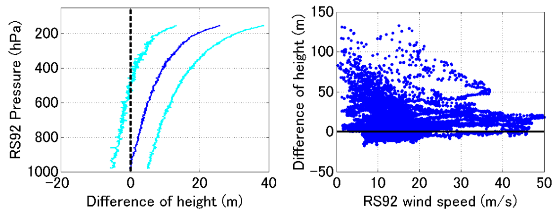
Figure 2.1-5: Mean difference of altitude between RS92-SGPD and RS41-SGP. Differences were calculated at the same observation time. Blue and cyan lines in the left panels denote mean difference and standard deviation.
