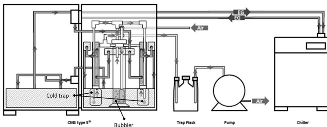
Figure 2.9-2: Schematic diagram of CMS type 5 th system
