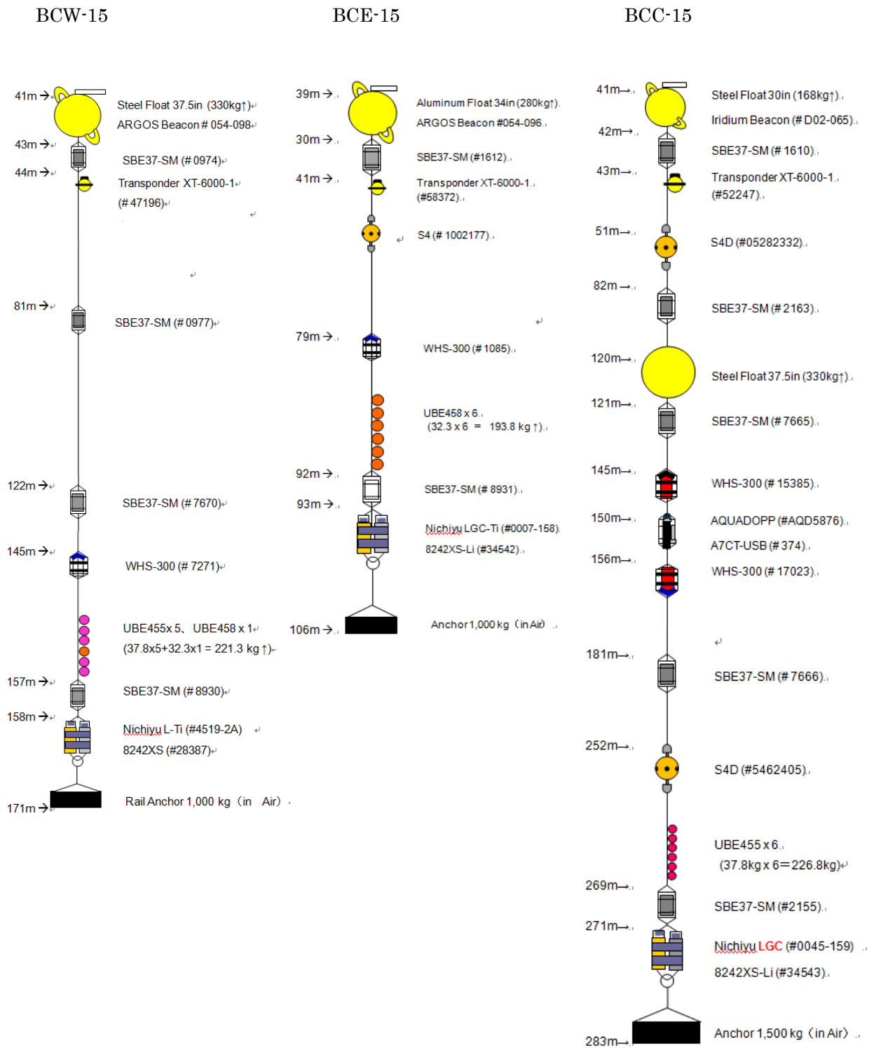
Figure 3.9-1: Diagrams of deployed moorings (BCW-15, BCE-15, and BCC-15).
