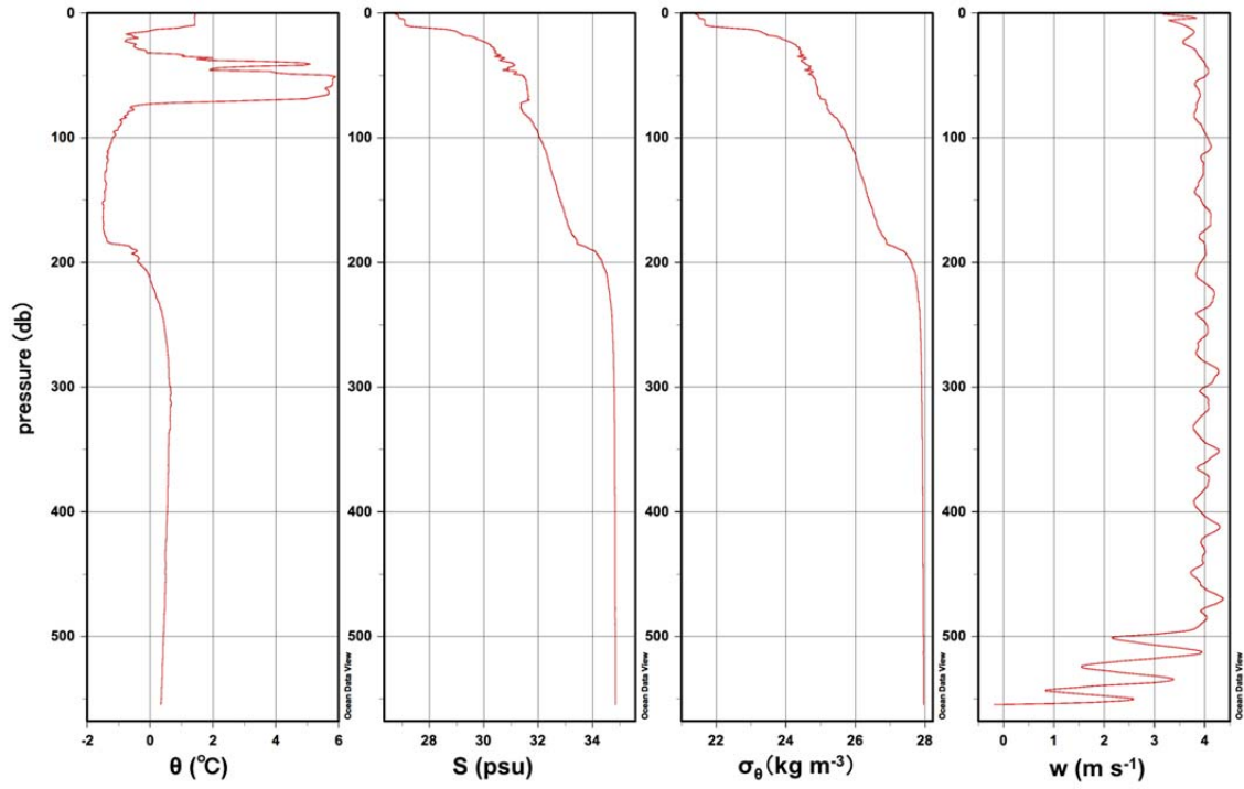
Figure 3.3-2: Typical profiles from U-CTD observation of (a) potential temperature \theta (deg-C), (b) salinity S (practical salinity unit), (c) potential density \sigma_\theta (kg m -3 ), and (d) descending rate w (m s -1 ) at a station of u003c01, positioned off the Barrow Canyon.
