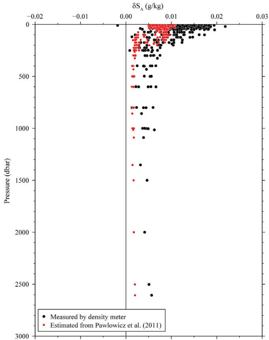
Figure 3.8-1: Vertical distribution of density salinity anomaly measured by the density meter. Absolute Salinity anomaly estimated from nutrients and carbonate parameters (Pawlowicz et al., 2011) are also shown for comparison.
