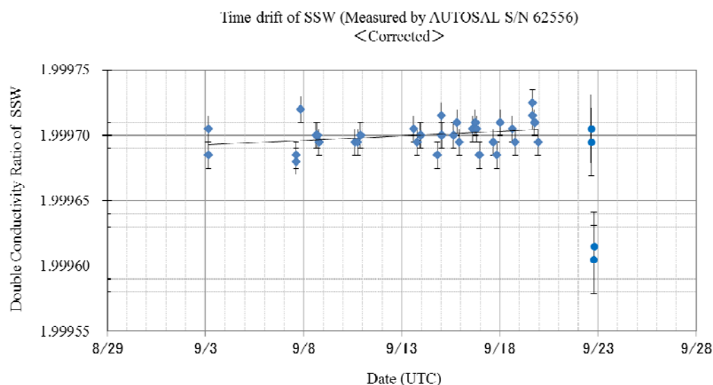
Fig. 3.7-2 History of double conductivity ratio for the Standard Seawater batch P157
