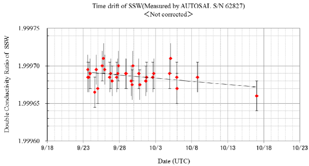
Fig. 3.7-3 History of double conductivity ratio for the Standard Seawater batch P157 in the salinometer S/N 62827 (before correction)
