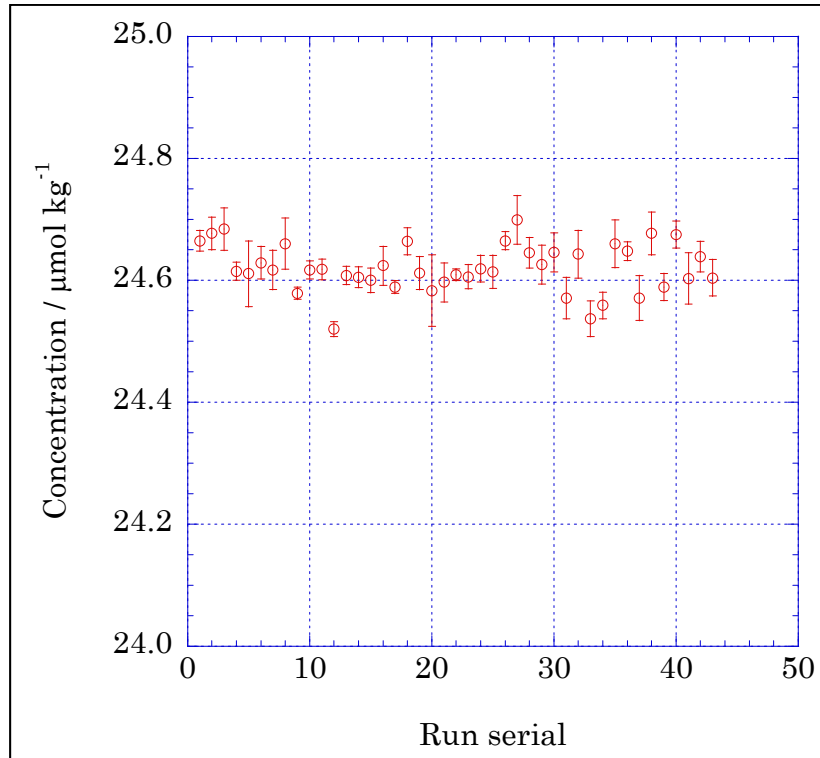
Figure 4.2-12 Time series of CRM-BW of nitrate in MR15-03.
