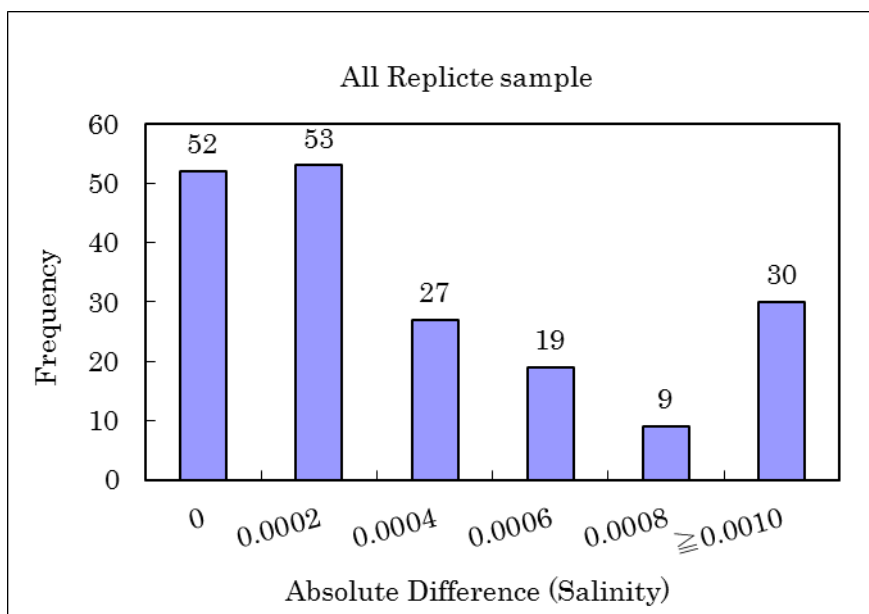
Fig. 3.7-5 Histogram of the Absolute Difference of all Replicate Samples
