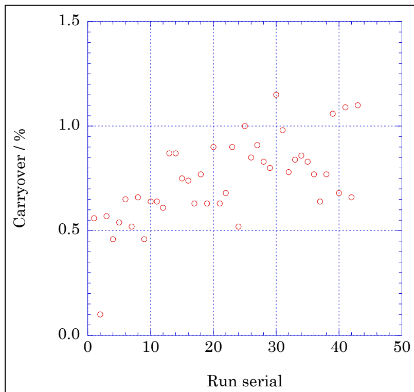
Figure 4.2-21 Time series of carry over of ammonia in MR15-03.
