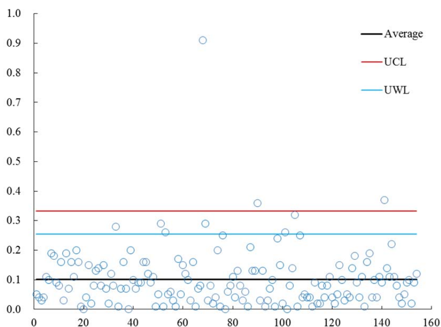
Fig. 4.1-1 Differences of replicate samples against sequence number
