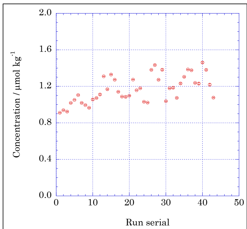
Figure 4.2-16 Time series of CRM-BW of ammonia in MR15-03.
