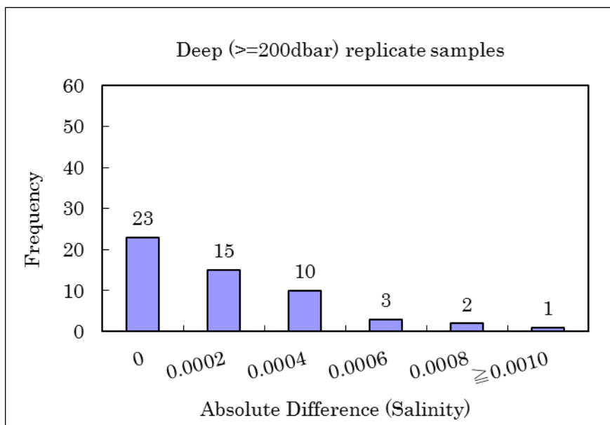
Fig. 3.7-7 Histogram of the Absolute Difference between Deep ( \geq 200 dbar) Replicate Samples
