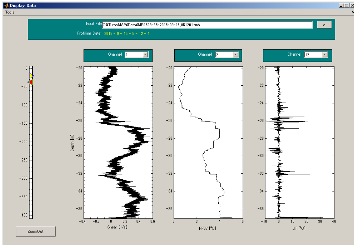
Figure 3.5-1: Vertical profiles of current shear, high-frequency temperature by FPO7, and vertical gradient of FPO7 temperature. The data were taken at (72-26.53°N, 156-36.01°W) at 05:12UTC September 15. A screen capture of a software TMTTools (JFE Advantech Co Ltd.).
