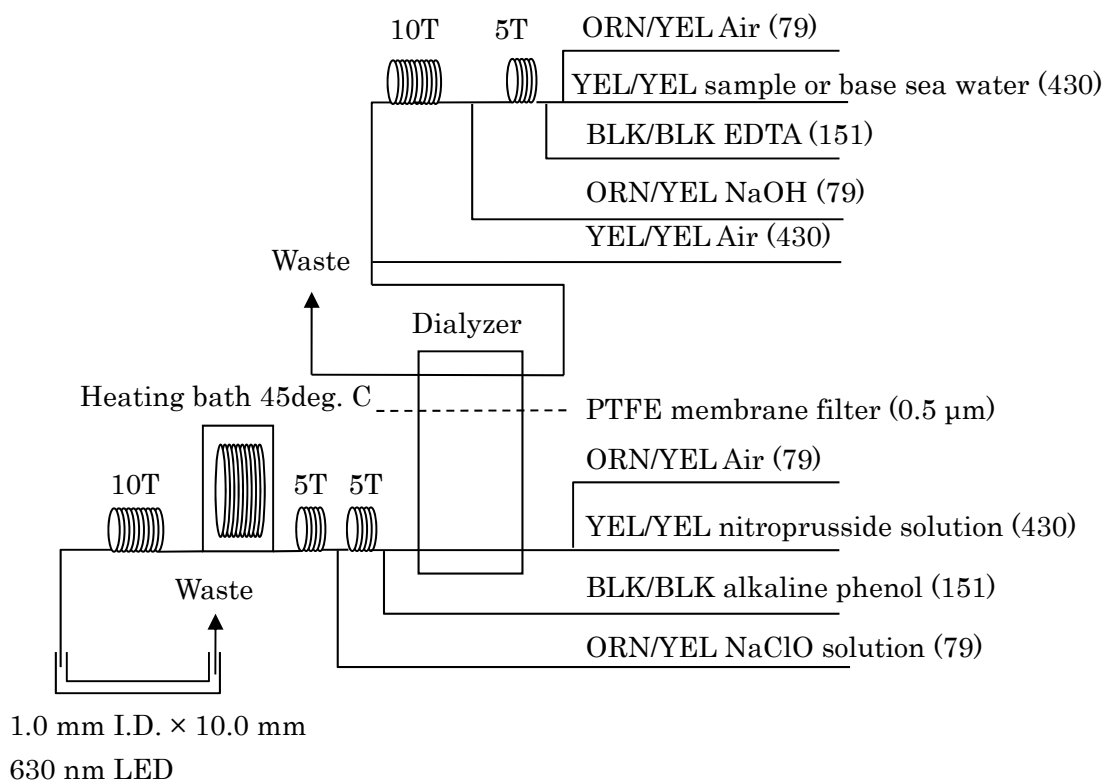
Figure 4.2-5 NH_4 (5ch.) Flow diagram.
