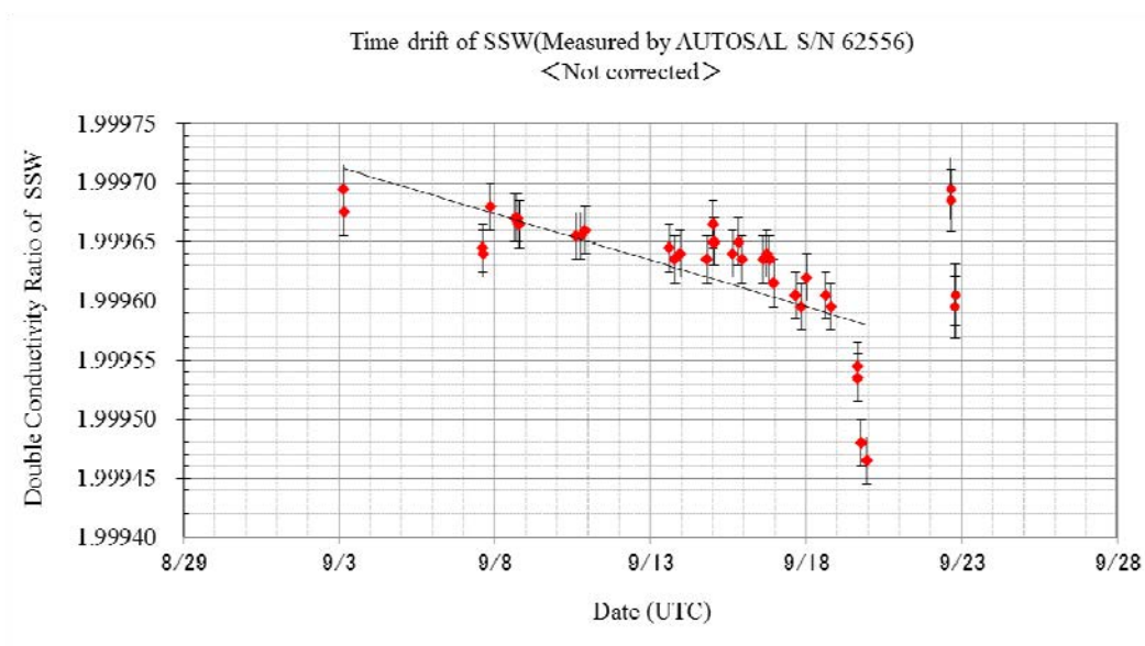
Fig. 3.7-1 History of double conductivity ratio for the Standard Seawater batch P157 in the salinometer S/N 62556 (before correction)
