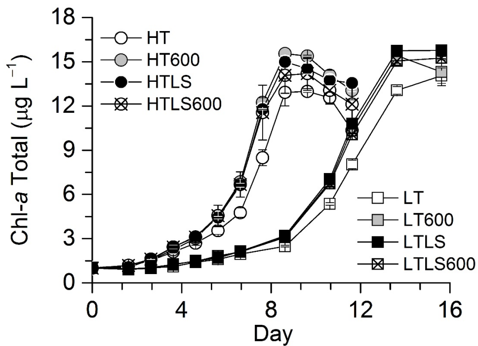
Fig. 4.19.2. Temporal change in chlorophyll- a concentration during the incubation.
