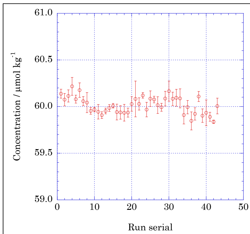
Figure 4.2-14 Time series of CRM-BW of silicate in MR15-03.
