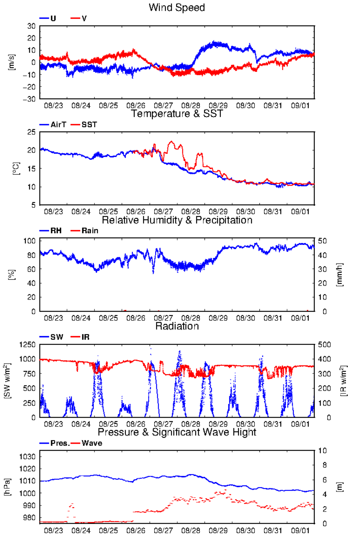
Figure 2.3-1: Time series of surface meteorological parameters during this cruise
