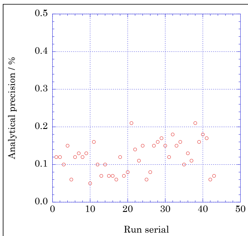
Figure 4.2-10 Time series of precision of phosphate in MR15-03.
