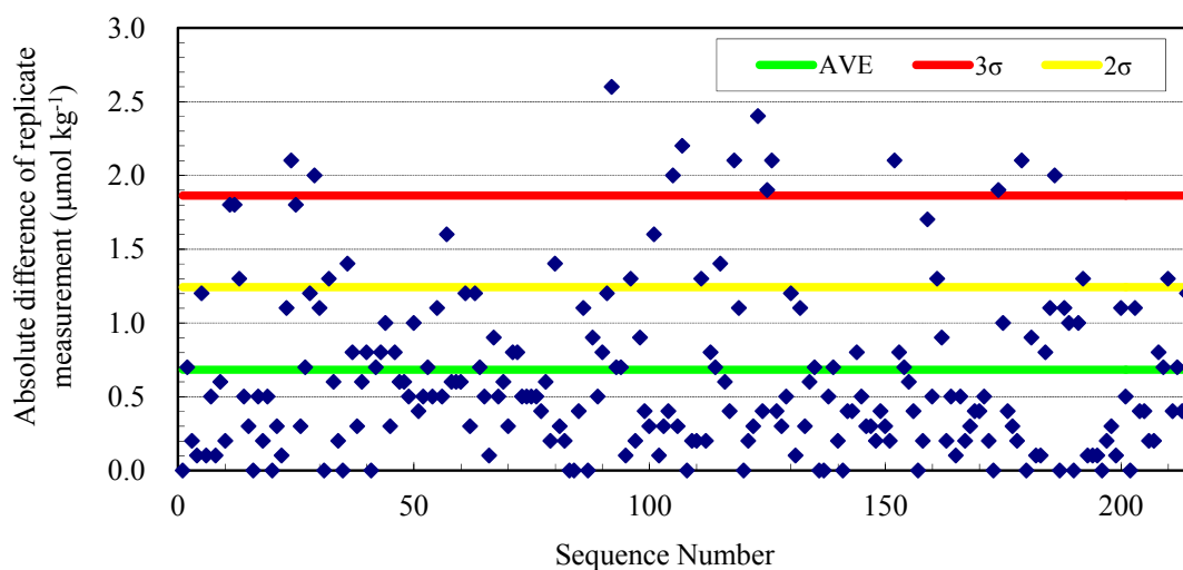
Figure 4.3.1-2 Range control chart of the absolute differences of replicate measurements carried out in the analysis of DIC during the MR15-03.
