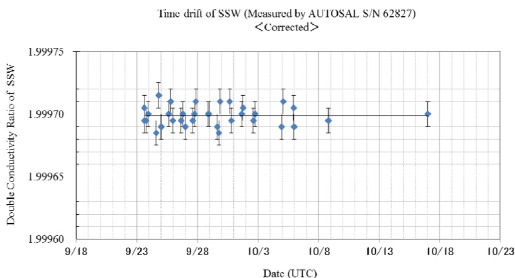
Fig. 3.7-4 History of double conductivity ratio for the Standard Seawater batch P157 in the salinometer S/N 62827 (after correction)
