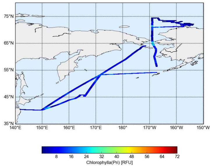
Figure 4.6-1: Spatial and temporal distribution of (a) temperature, (b) salinity, (c) dissolved oxygen, and (d) fluorescence in MR15-03 cruise.
