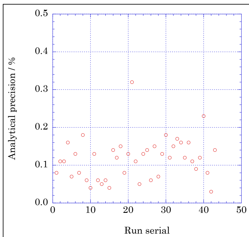
Figure 4.2-9 Time series of precision of silicate in MR15-03.
