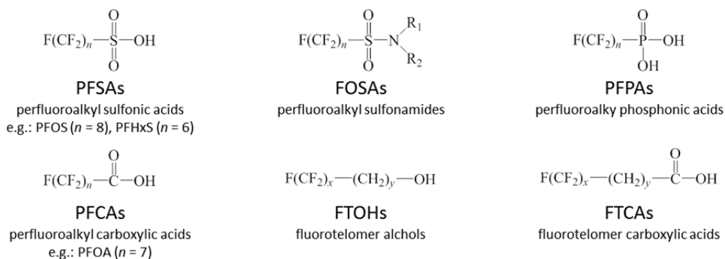
Figure 2.9-1: Perfluoroalkyl substances (PFASs)
