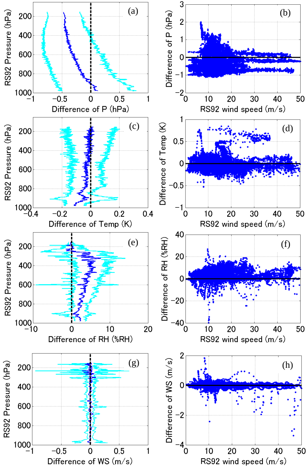
Figure 2.1-4: Mean differences of (a, b, i, j) pressure, (c, d, k, l) temperature, (e, f, m, n) relative humidity, and (g, h, o, p) wind speed between RS92-SGPD and RS41-SGP. Differences were calculated at the same (a-h) observation time or (i-p) altitude. Blue and cyan lines in the left panels denote mean difference and standard deviation.
