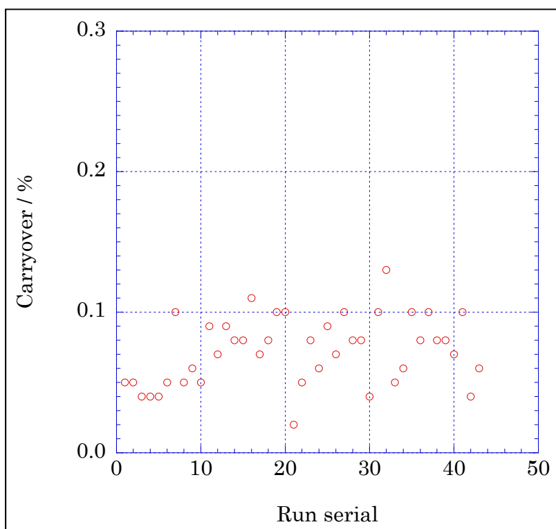
Figure 4.2-19 Time series of carry over of silicate in MR15-03.
