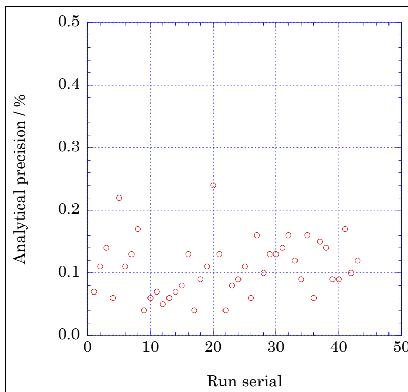
Figure 4.2-7 Time series of precision of nitrate in MR15-03.
