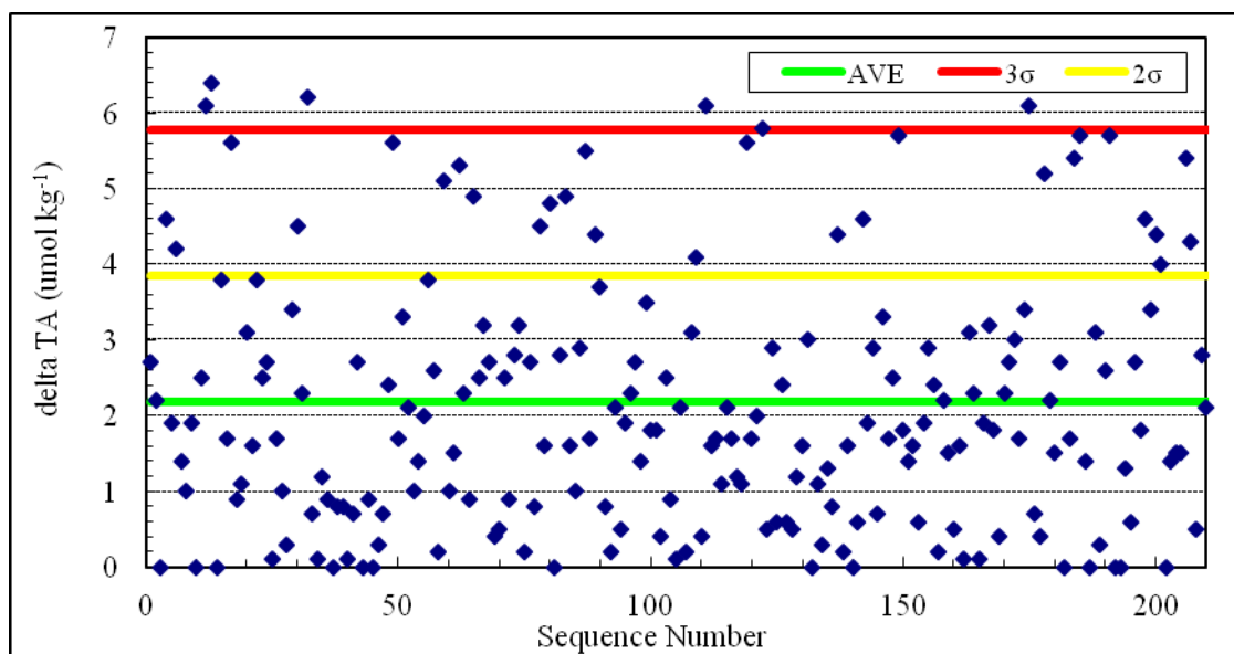
Figure 4.4-3 Range control chart of the absolute differences of duplicate measurements of TA carried out during this cruise.
