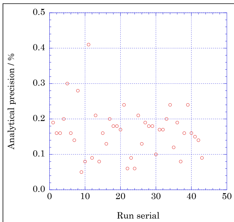
Figure 4.2-8 Time series of precision of nitrite in MR15-03.
