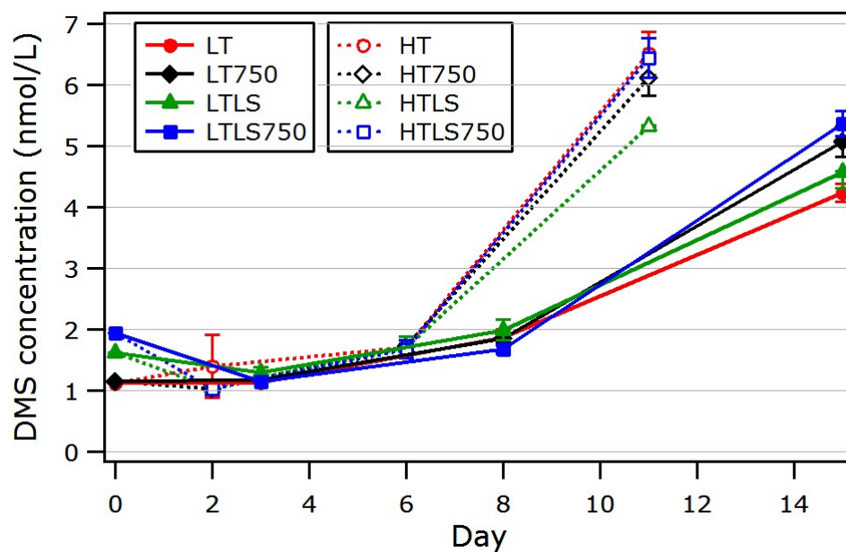
Figure4.8-2: Time series of DMS concentrations during incubation experiment.
