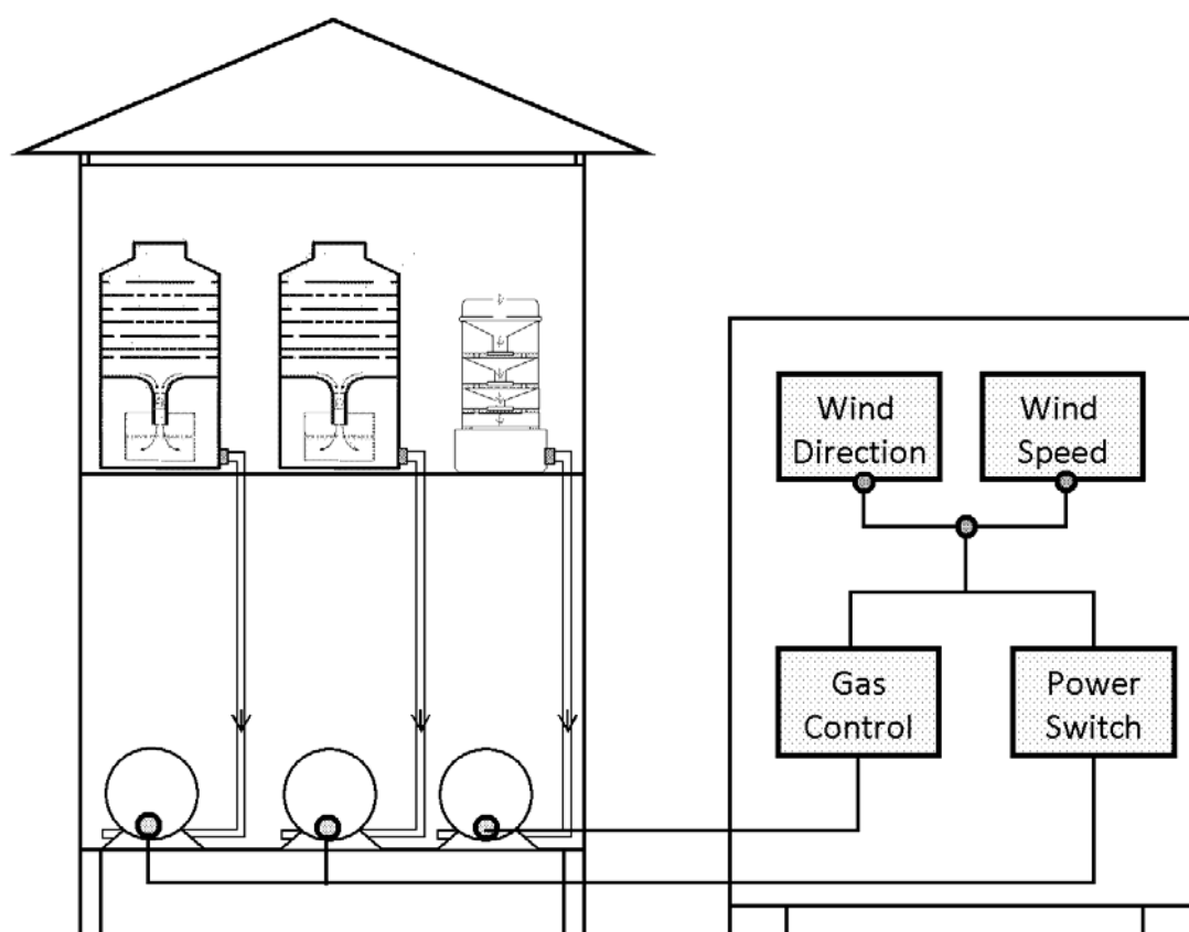
Figure 2.9-3: Schematic diagram of Cascade impactor sampling system
