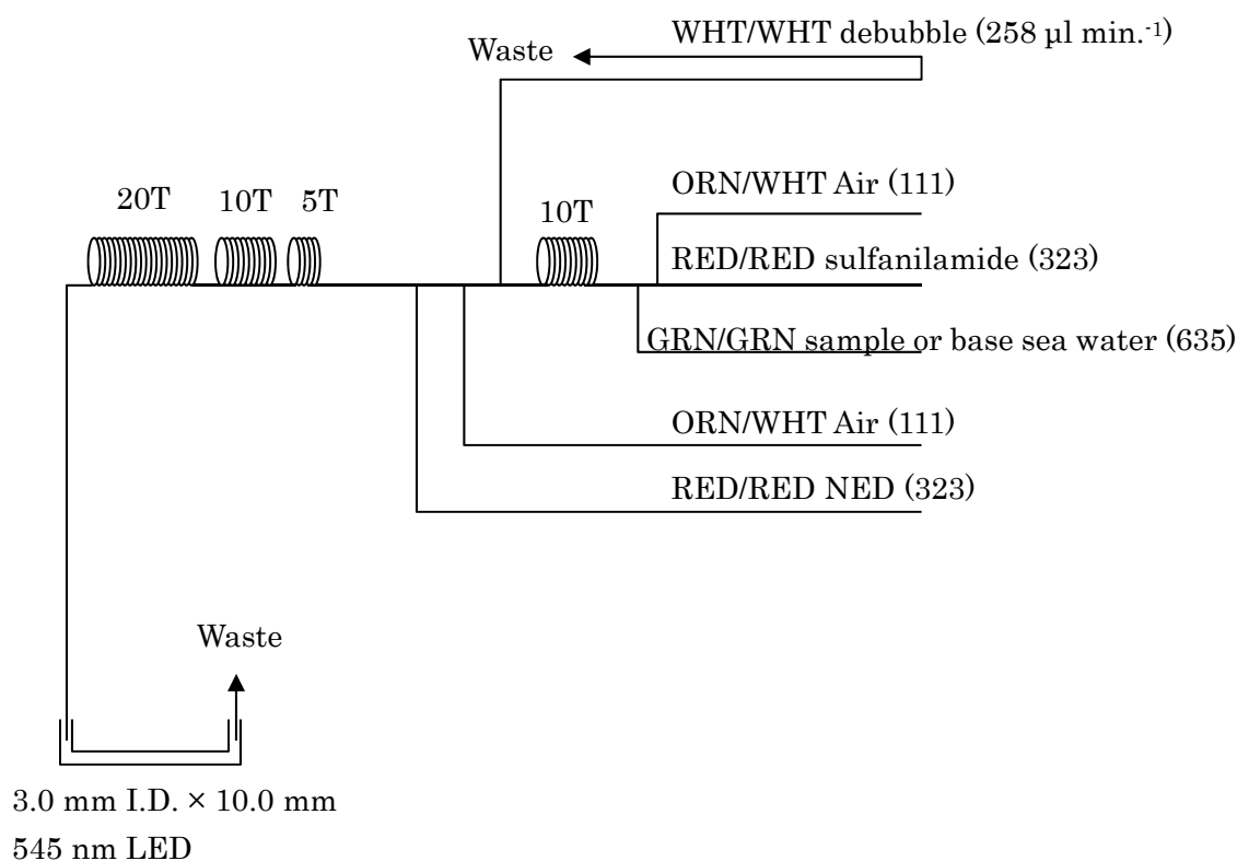
Figure 4.2-2 NO 2 (2ch.) Flow diagram.
