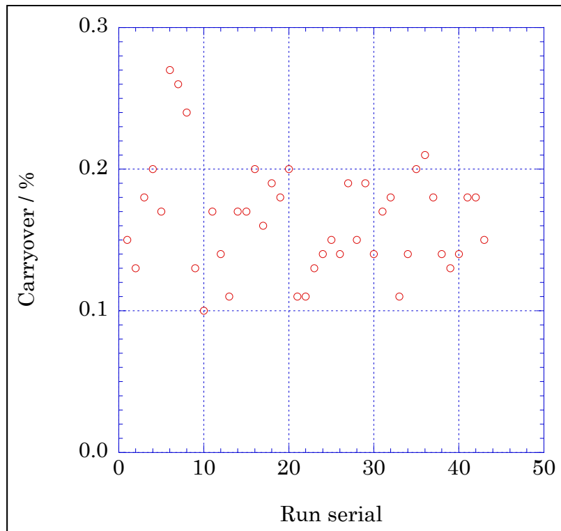
Figure 4.2-20 Time series of carry over of phosphate in MR15-03.
