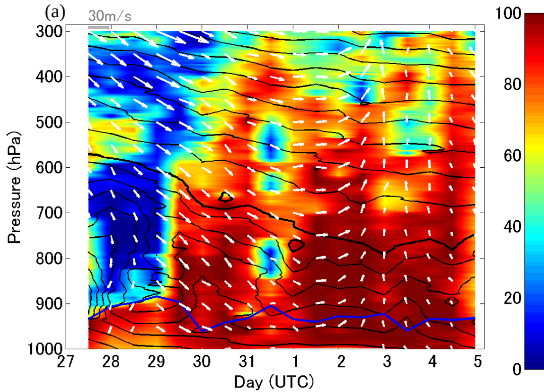
Figure 2.1-2: Time-height section of relative humidity (color), air temperature (black contours) and wind (vectors). Black bold contour denotes 0 °C. Contour interval is 5 °C (2 °C) when the temperature is less (more) than 0 °C. Blue contour shows the mixed layer height defined as the height where potential temperature is higher by 2.0 °C than the surface. (a) 27 August – 5 September (leg 1, every 12 hours), (b) 6–20 September (leg 1, every 6 hours), (c) 21 September – 5 October (leg 1, every 6 hours), and (d) 11–20 October (leg 2, every 12 hours).
