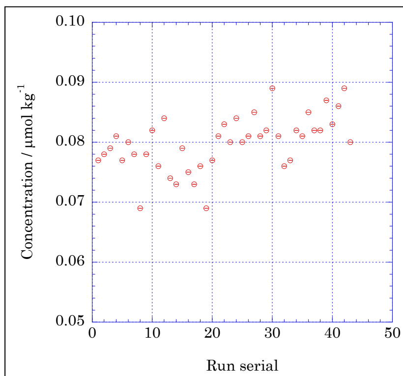
Figure 4.2-13 Time series of CRM-BW of nitrite in MR15-03.
