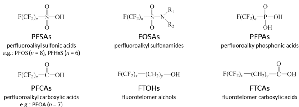
Figure 4.9- 1 Perfluoroalkyl substances (PFASs)
