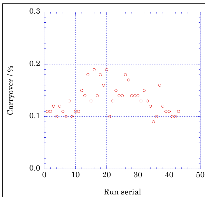
Figure 4.2-17 Time series of carry over of nitrate in MR15-03.
