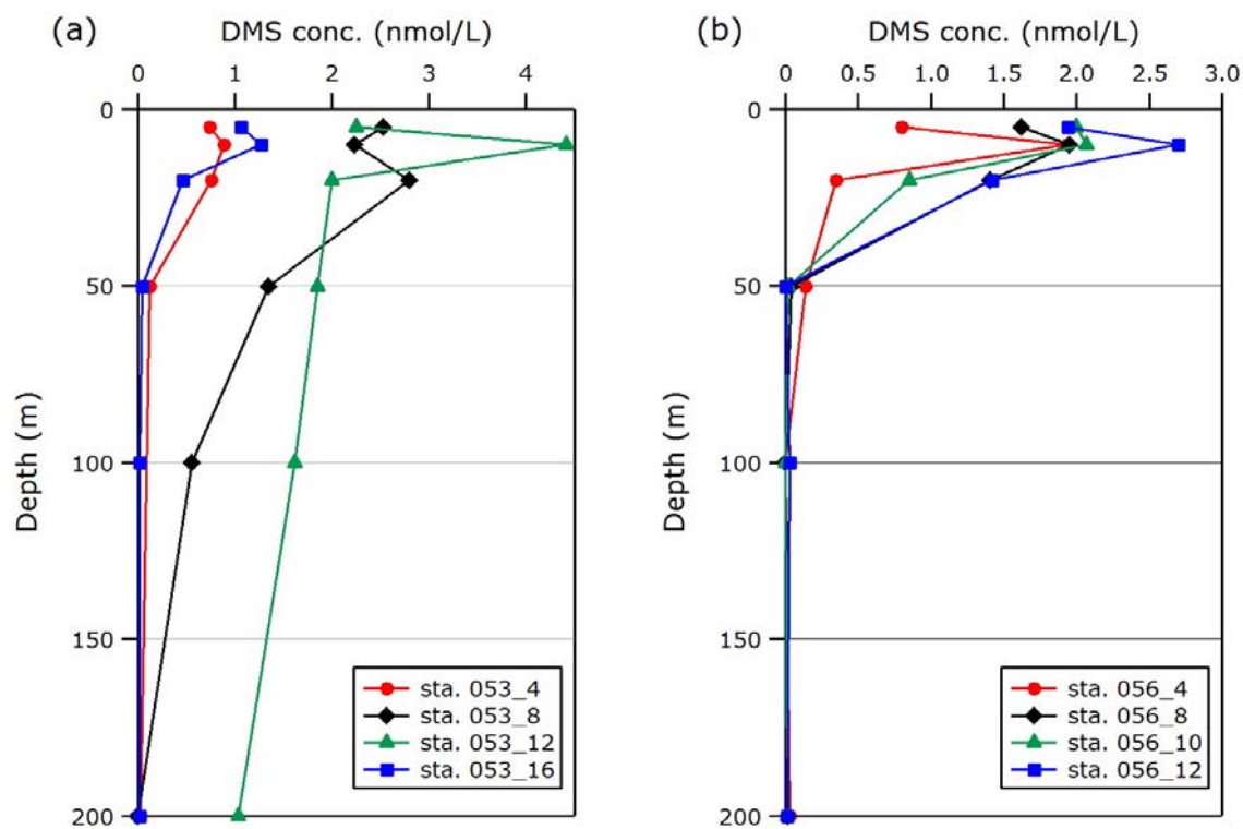
Figure4.8-1: Vertical distribution of DMS concentration during fixed point observations in (a) sta. 053 and (b) sta. 056.
