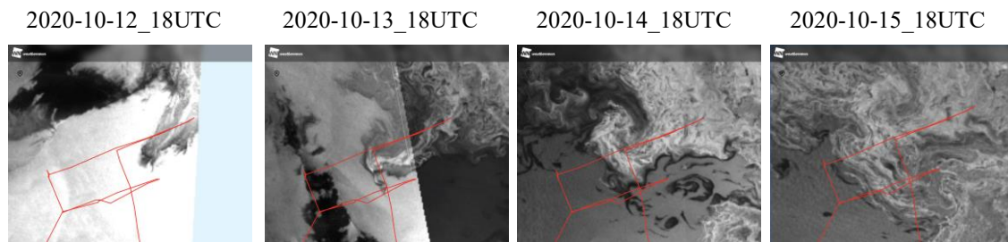
Figure 2.4-3. Marginal ice zone eddy development. Red line is MIRAI ship track.
