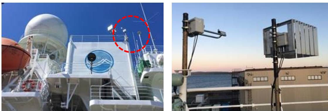
Figure 2.5.4-1. Onboard LPM sensors. (Left) The location of the sensors, as designated by the red broken circle. (Right) The sensors. Right one (aft one) equipped wind protection element to reduce the effect of the wind, while left one (fore one) did not.
