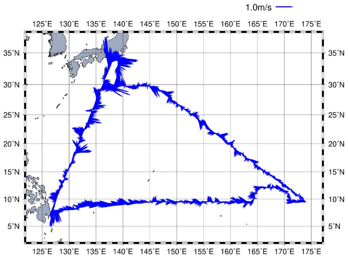
Fig. 3.5-2 Horizontal Velocity along the ship's track. (15 min. Average / Layer: 39-55 m)
