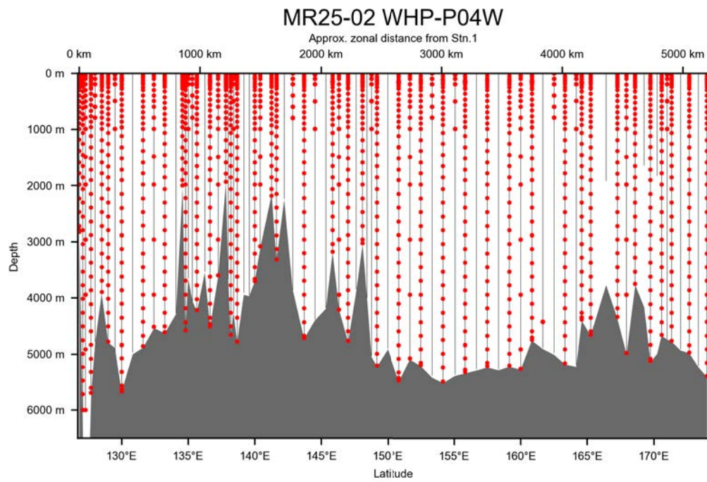
Fig. 1.2. Cross sections showing data sampling positions. Black line shows CTD trace and
