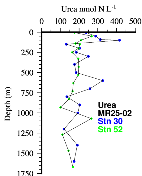
Figure 4.19.1: Preliminary data for Urea ( \text{nmol N L}^{-1} ) at stations 30 and 52 during MR25-02.
