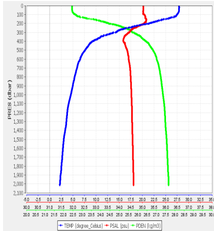
Fig. 5.1.2 (c). Vertical temperature, salinity and density profiles of their first measurements for two Core Argo floats (SN10800 and SN 10801). Blue, red and light green lines show temperature, salinity and density profiles.
