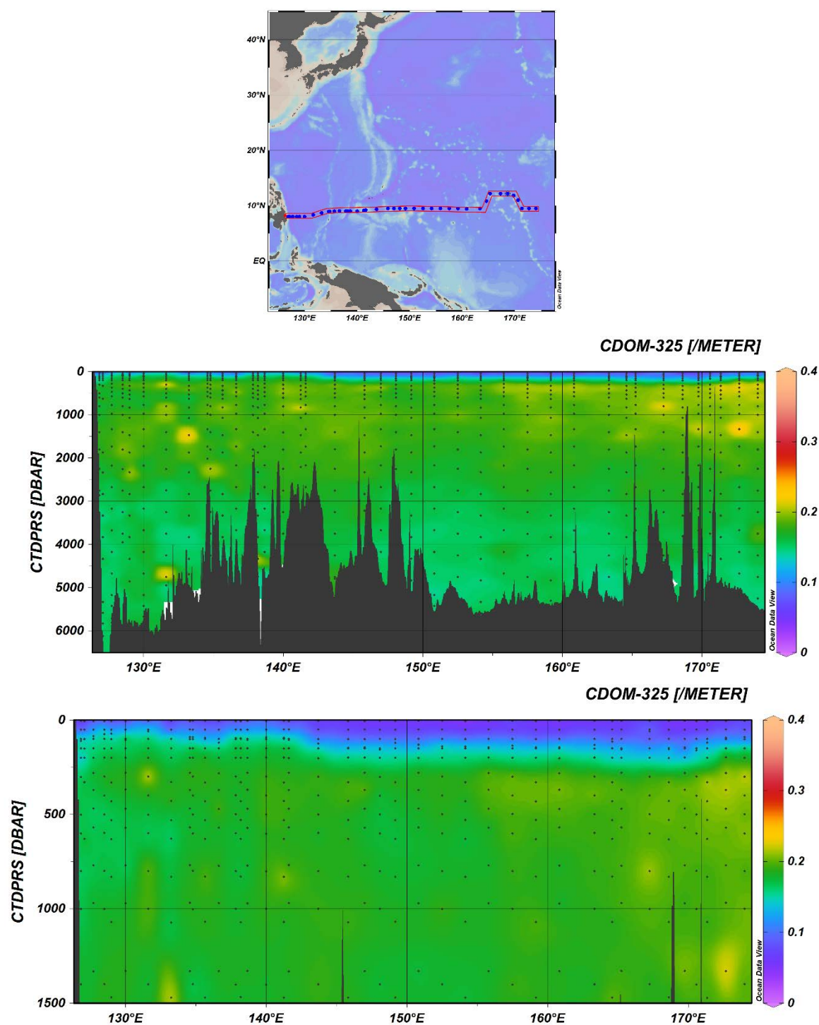
Fig.4.14.2 Sections of CDOM (as absorption coefficient at 325 nm, unit = \text{m}^{-1} ) along P04W section obtained from hydrographic casts. The top section covers surface to the bottom and the lower section covers the upper 1,500 m.
