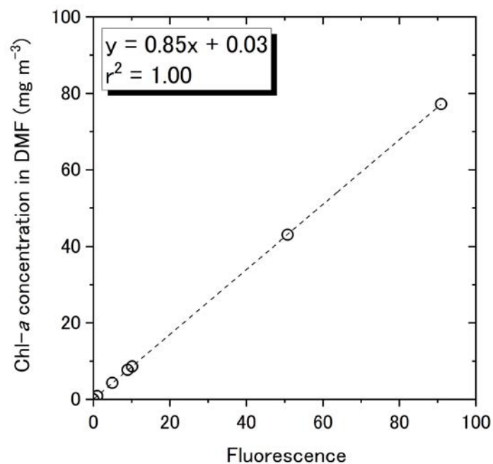
Figure 4.11.1 Relationships between pure chlorophyll a concentrations and fluorescence light intensity (n=7).
