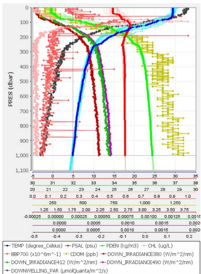
Figure 5.2.1. Vertical profiles of the first measurements.
