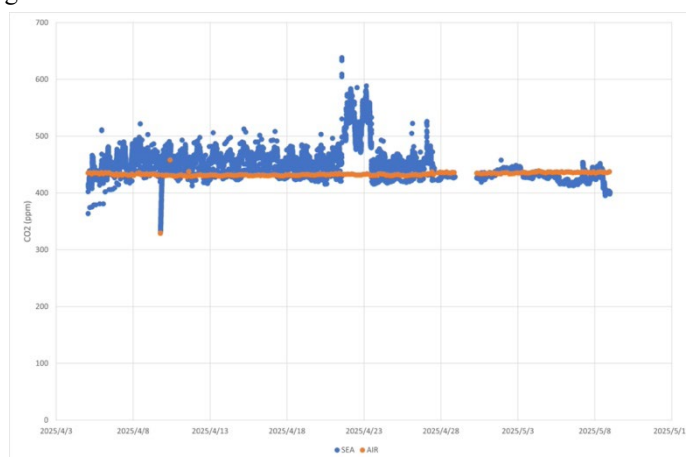
Fig. 3.10-1 Distributions of atmospheric (orange) and surface seawater CO 2 (blue) along the observation line as a function of time
