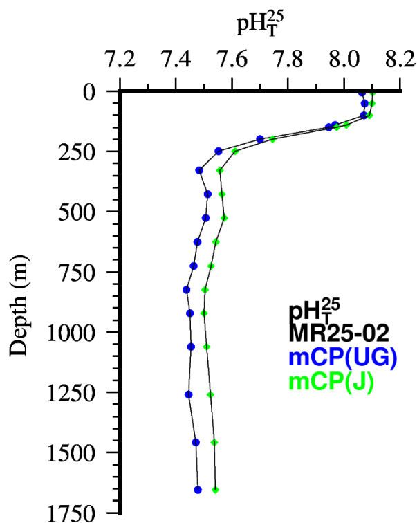
Figure 4.20.2: Vertical profiles of \text{pH}_T^{25} (preliminary data) at station 52 during MR25-02 using the University of Galway analytical system (1 cm pathlength). The blue circles were with the purified mCP supplied by the University of Galway, the green triangles are with the purified mCP supplied by JAMSTEC. No corrections have been applied yet for the dye addition.
