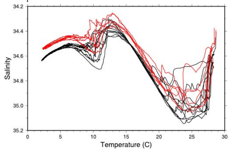
Figure 4.26-2. Temperature-salinity relationships for the CTD (black lines) and the XCTD (red lines) obtained between the stations 64 and 76. The data for depths shallower than 2000 m were plotted.
