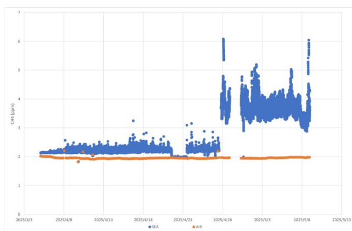
Fig. 3.10-2 Distributions of atmospheric (orange) and surface seawater CH 4 (blue) along the observation line as a function of time
