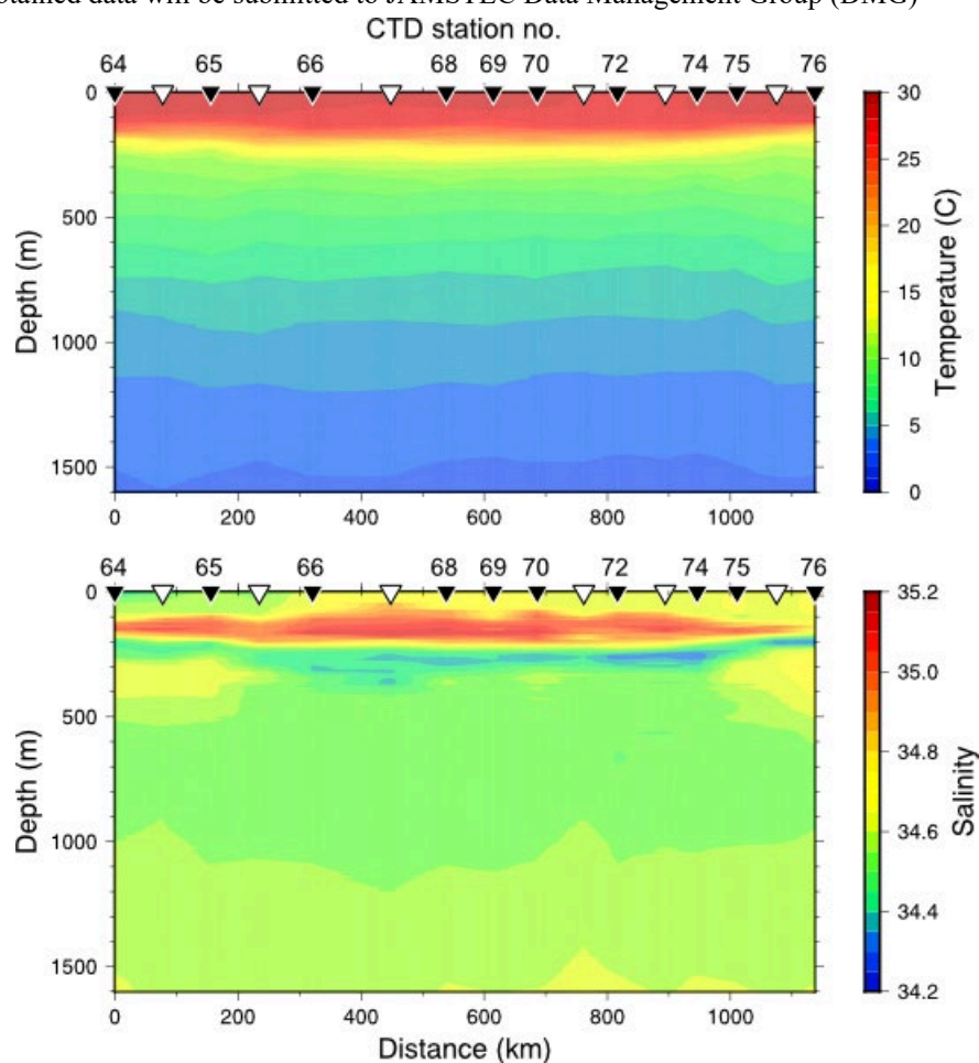
Figure 4.26-1. Vertical sections of temperature (upper) and salinity (lower) obtained by the CTD and
