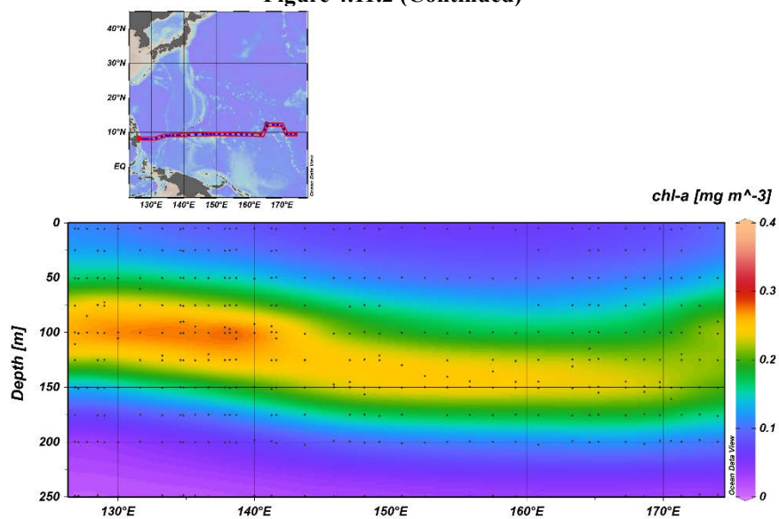
Figure 4.11.3 Cross section of chlorophyll a concentrations along the P04W section (upper map) obtained from hydrographic casts.
