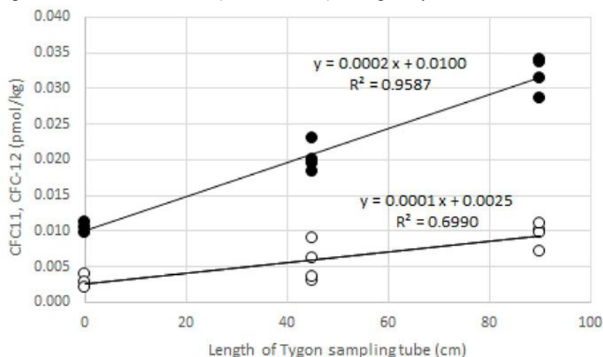
Fig. 4.8.2 Estimate of contamination of CFC-11 and CFC-12 from the Tygon sampling tube.
