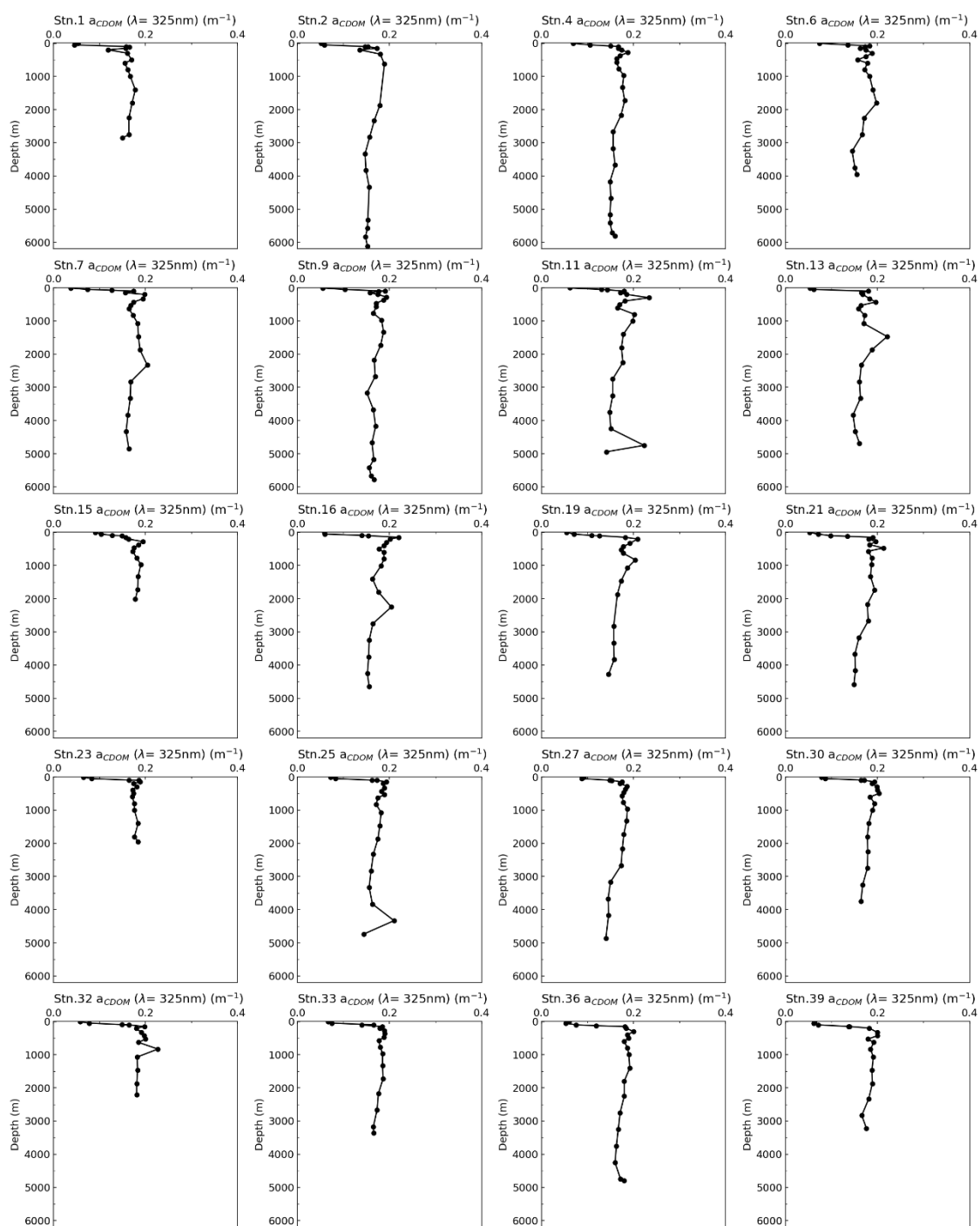
Fig.4.14.1 Vertical profiles of CDOM (as absorption coefficient at 325 nm, unit = \text{m}^{-1} ) at all sampling stations.
