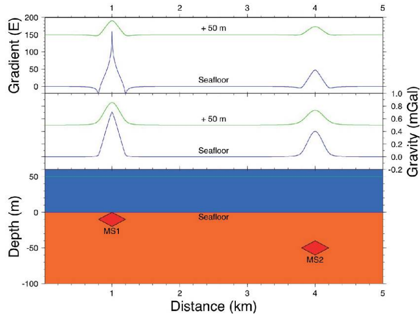
Fig.2 Estimated gravity (middle) and gradient (upper) variations are on a model (bottom). The model has two same shape deposits, MS1 and MS2, which have density differences of 1 \text{ g/cm}^3 against background.
