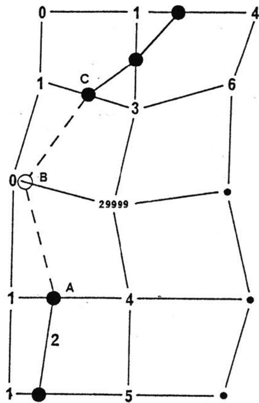
図3 航跡に沿ったデータ点(欠測点を含む)とそれに基づく等深線作画 Fig. 3 Distribution of data points along the ship track (including dummy data) and contouring procedure based on the data points.
