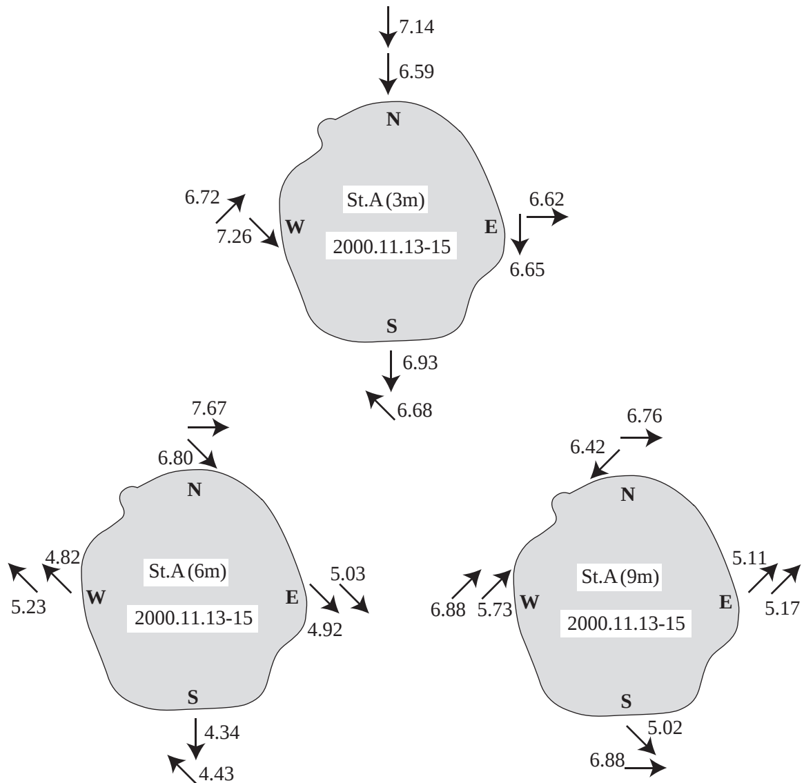
図4 St.A近傍における流れの概略図 (2000.11.13~15) Fig. 4 Schematic view of water motion at St.A during Nov. 13th - 15th, 2000.
