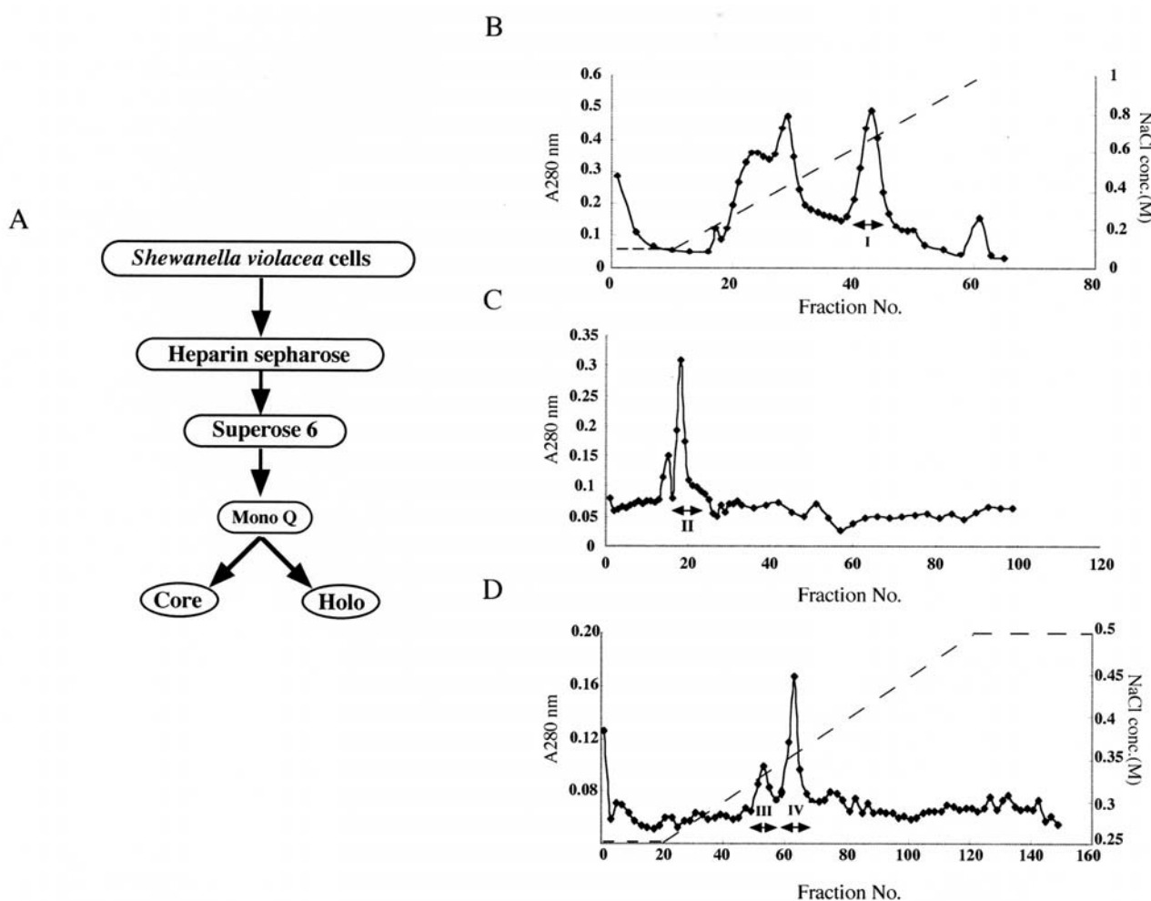
Fig. 1 Purification of S. violacea RNA polymerase.
