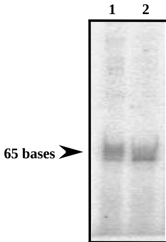
Fig. 3 In vitro transcription with RNA polymerase of S. violacea and E. coli .
