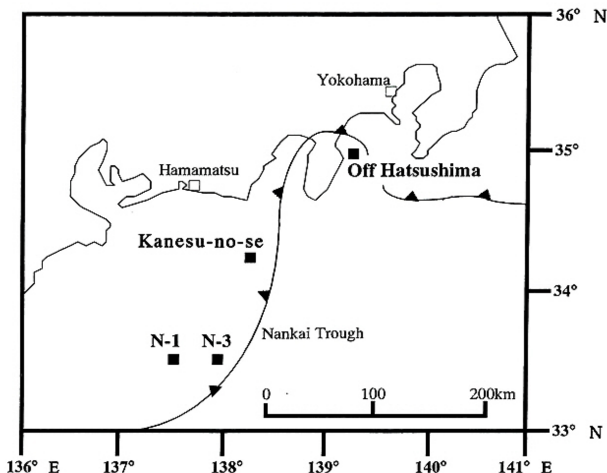
図1 堆積物試料の採取地点 Fig. 1 Sites of sediment sample collection
