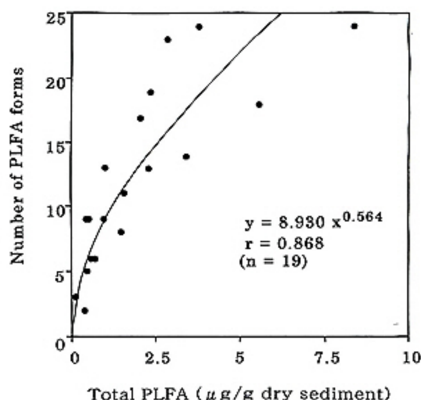
図2 堆積物中のリン脂質脂肪酸含量と脂肪酸種数の関係 Fig. 2 Correlation between contents and numbers of phospholipid fatty acids (PLFA) extracted from sediment samples.
