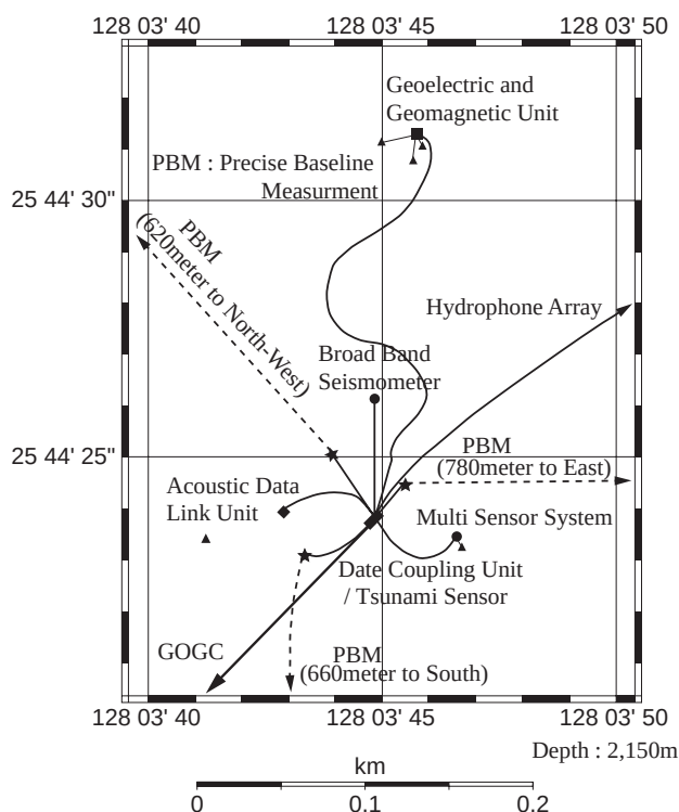
Fig. 4 Geographical arrangements for instruments of MDOBO, DCU and SMCC at the VENUS site.
