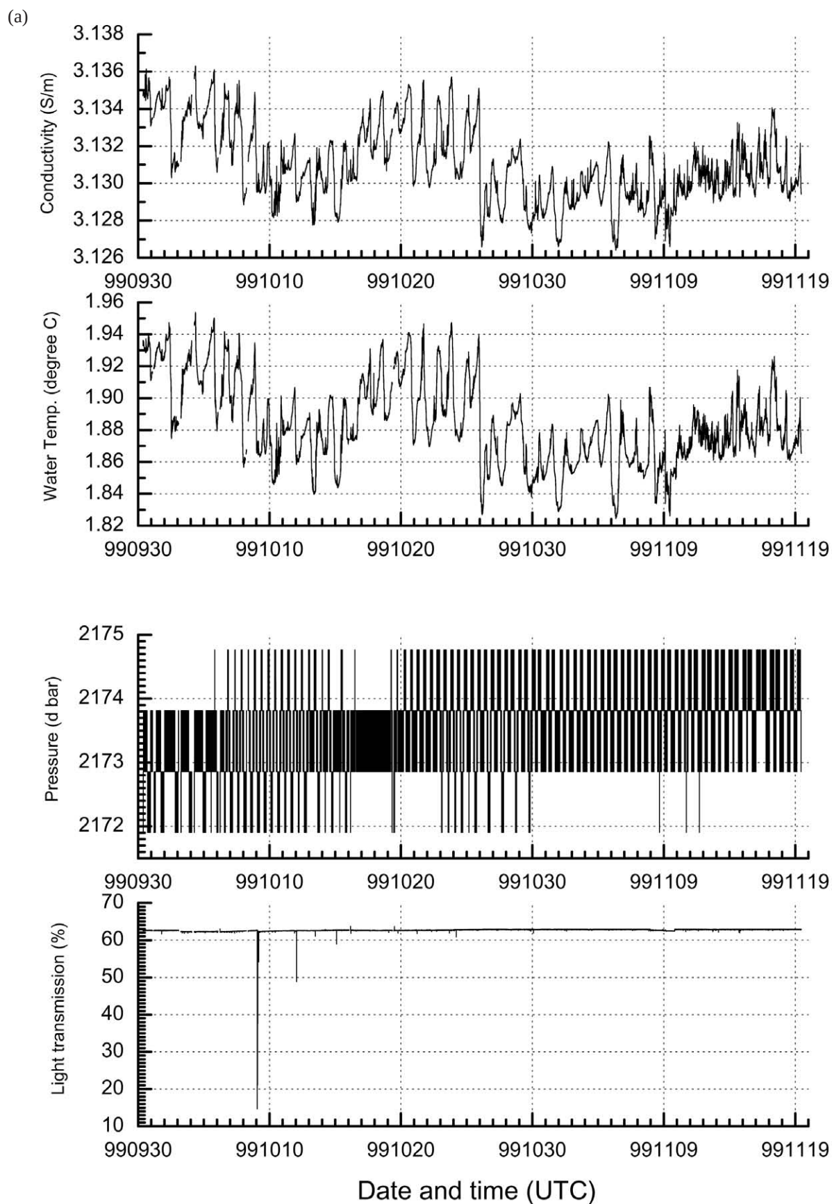
Fig. 11 Records obtained by the multi-sensor system. (a) Electrical conductivity, water temperature, water pressure and light transmission through water.
