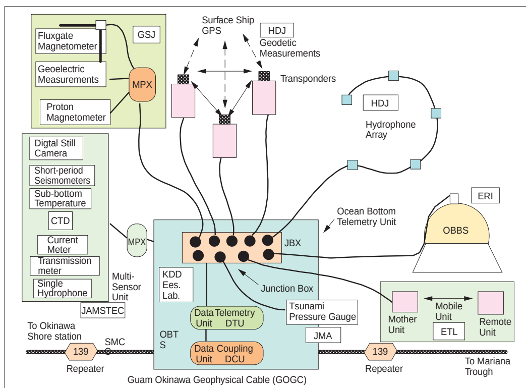
Fig. 3 The VENUS ocean bottom system (SMCC, DCU, DTU, JBX and MDOBO) developed by multi-institutions. Abbreviations are the same as the ones in Fig. 2.
