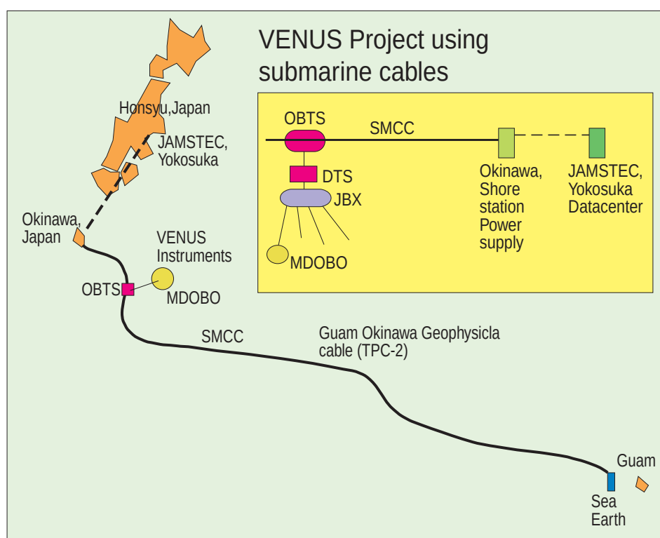
Fig. 2 The VENUS system from the MDOBO to the data center in Yokosuka. MDOBO: Multi-Disciplinary Ocean-Bottom Observatory; JBX: Junction BoX; DTS: Data Telemetry System; OBTS: Ocean Bottom Telemetry System and SMCC: Sub-Marine Coaxial Cable.
