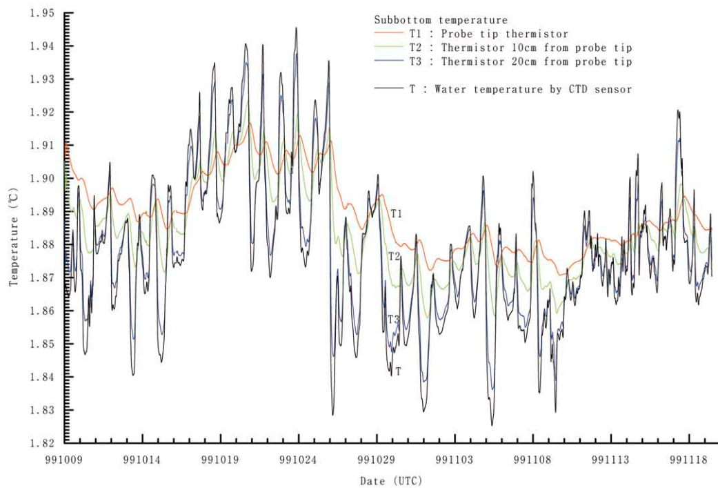
Fig. 11 Records obtained by the multi-sensor system.
