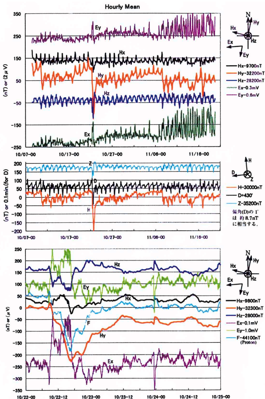
Fig. 10 Records of geo-magnetic and geo-electrical measurements. 42 days observation at the deep-sea site (top) and data from Kakioka magnetic observatory (middle) reveal a good correlation with a slight difference due to the difference in latitudes. Variation of the magnetic storm on Oct. 22, 1999 (JST) and its succeeding phenomena are shown on the bottom. The electrical field disturbance became larger after Nov. 6, 1999, which might indicate some unknown process related with the abrupt termination of the VENUS system.
