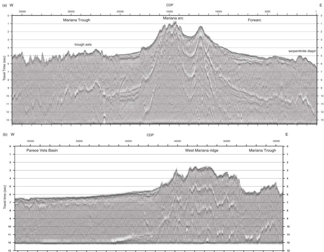
Fig. 9 MCS profile. (a) Eastern half obtained by KY03-01 cruise. (b) Western half obtained by KY03-06 cruise.
