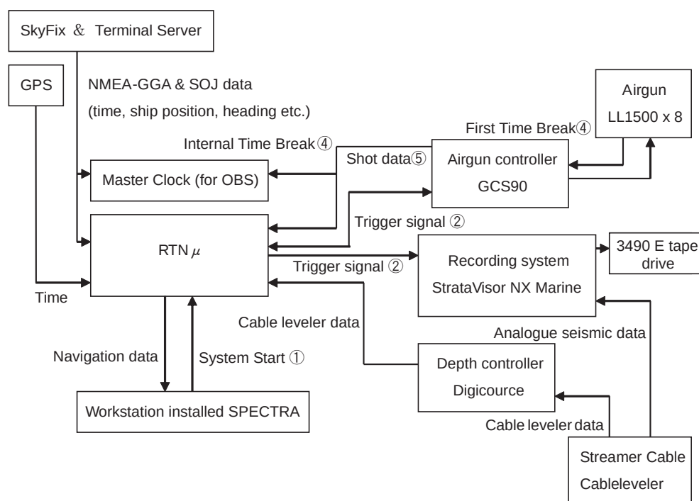
Fig. 3 Flow chart of the MCS recording system. Circled numerals show the timing flow of this seismic system.
