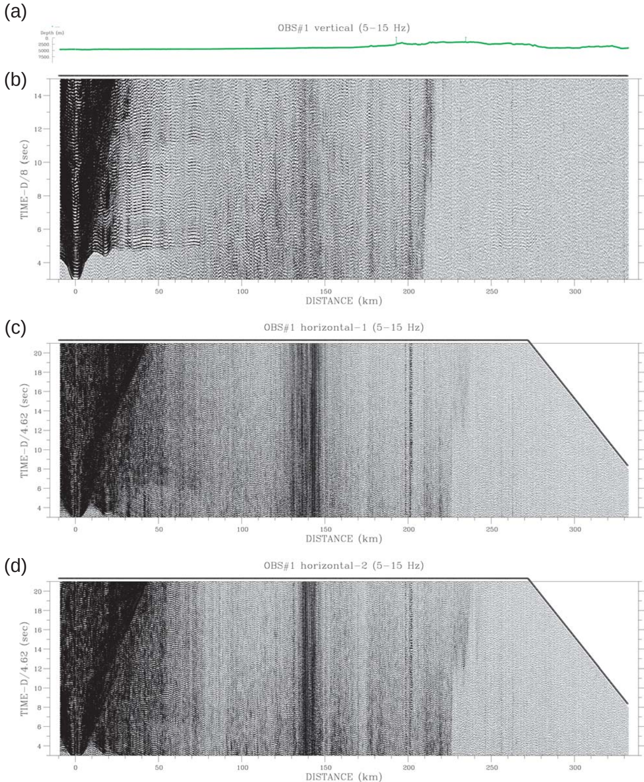
Fig. 4 Record sections of OBS#1. All traces are filtered by 5-15 Hz. Horizontal and vertical axes are offsets from OBS and reduced traveltimes by 8 km/s for vertical component or 4.62 km/s for horizontal components. (a) Topography. (b) Vertical component. (c) Horizontal-1 component. (d) Horizontal-2 component.
