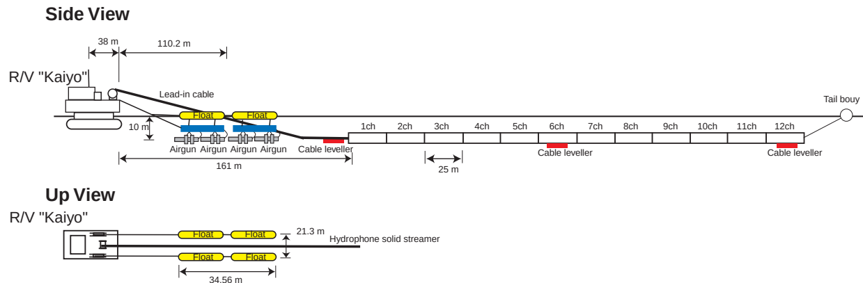
Fig. 2 Geometry of seismic experiment.
