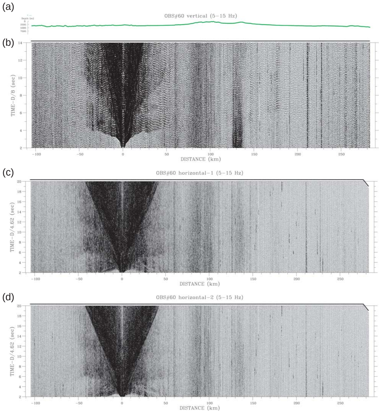
Fig. 6 Record sections of OBS#60. The details are same as for Figure 4. (a) Topography. (b) Vertical component. (c) Horizontal-1 component. (d) Horizontal-2 component.
