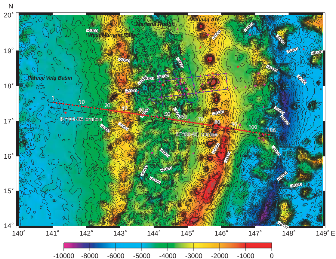
Fig. 1 Map of the experimental area. Solid circles indicate OBSs and available OBSs are shown by red circles. We shot an airgun array on a thick black line. Red and purple stars indicate the long term OBSs for natural earthquake observations. Blue lines indicate airgun shooting lines for the long term OBSs.
