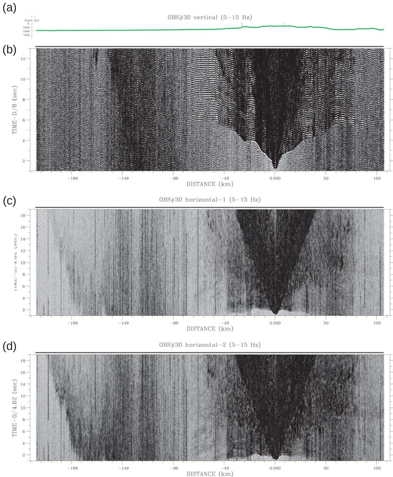
Fig. 5 Record sections of OBS#30. The details are same as for Figure 4. (a) Topography. (b) Vertical component. (c) Horizontal-1 component. (d) Horizontal-2 component.
